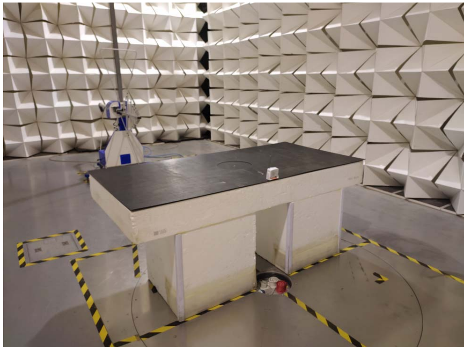
Radiated Emission 30MHz to 1GHz
