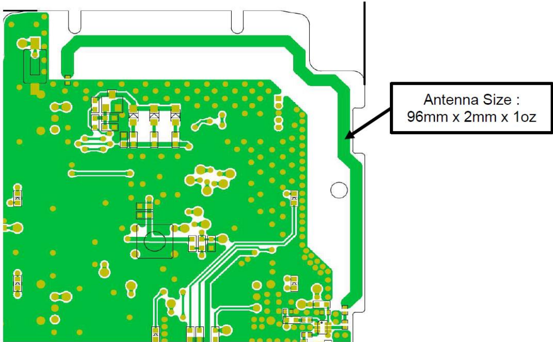
NGM-41-FSK Antenna
