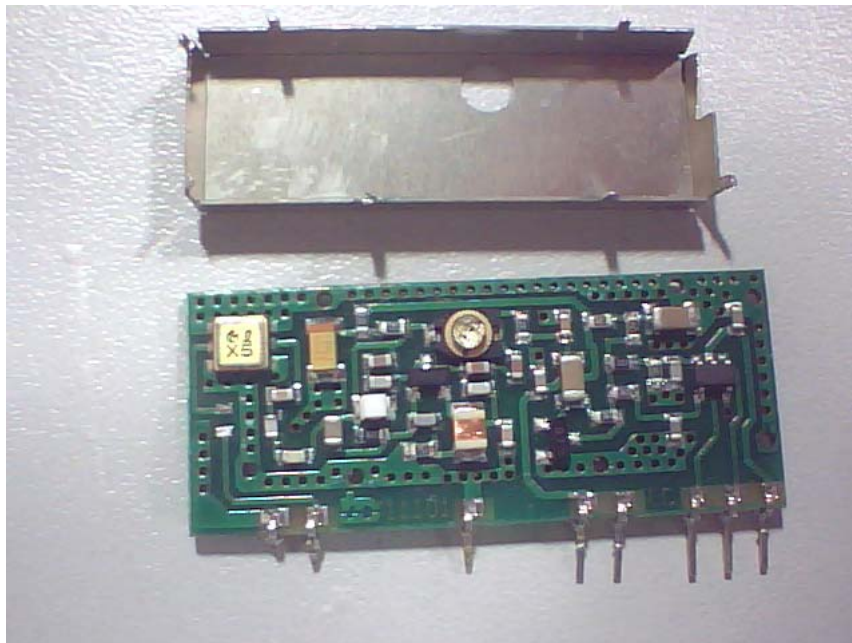
PCB Front View of Receiver Module
