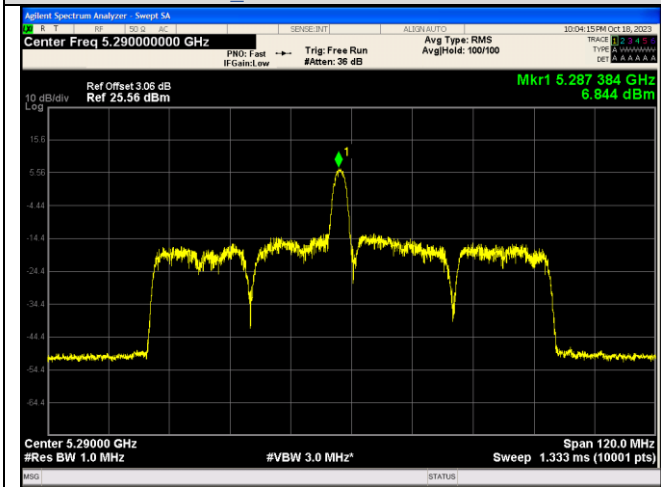
IEEE 802.11ax_Channel 58_80MHz_Antenna 2_RU&Index 26RU17
