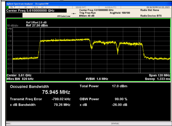
IEEE 802.11ax_Channel 122_80MHz_Antenna 2_RU&Index 484RU65
