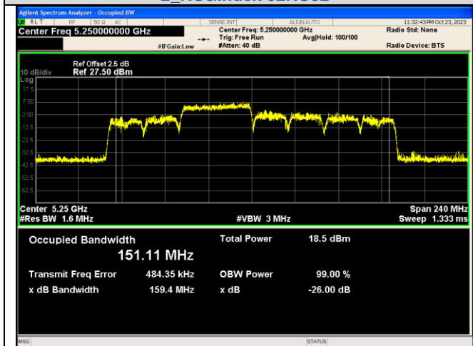
IEEE 802.11ax_Channel 50_160MHz_Antenna 2_RU&Index 484RU66
