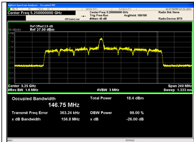
IEEE 802.11ax_Channel 50_160MHz_Antenna 2_RU&Index 52RU52
