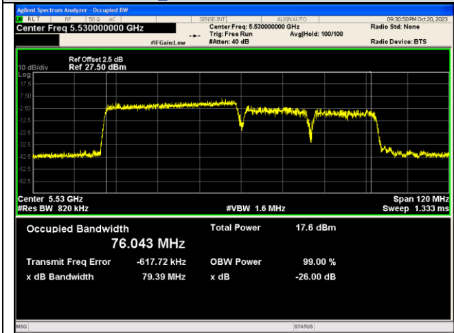
IEEE 802.11ax_Channel 106_80MHz_Antenna 2_RU&Index 484RU65
