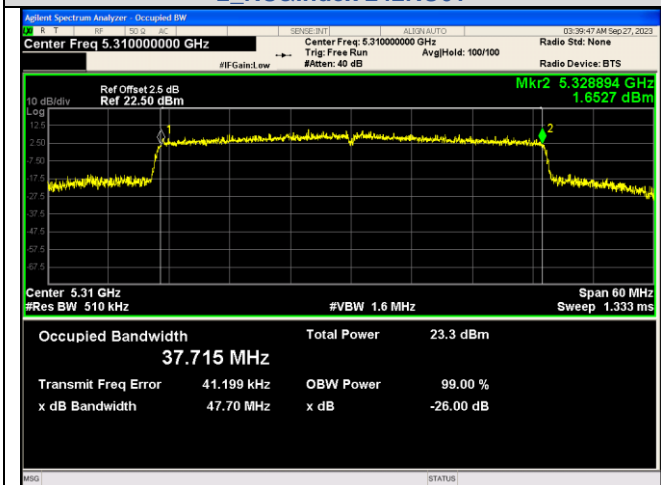
IEEE 802.11ax_Channel 62_40MHz_Antenna 2_RU&Index 484RU65
