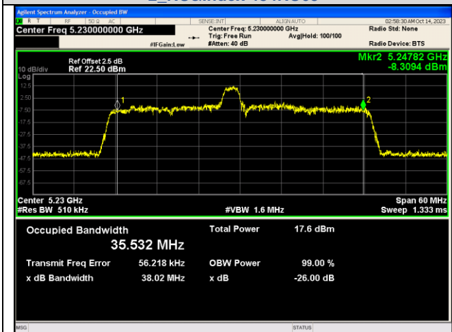
IEEE 802.11ax_Channel 46_40MHz_Antenna 2_RU&Index 26RU8
