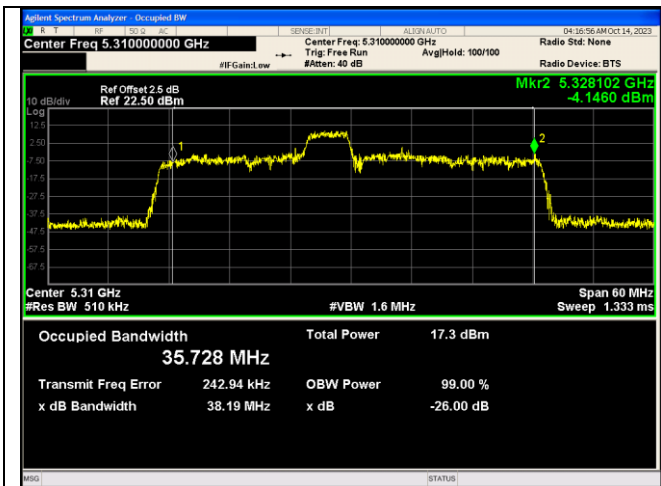
IEEE 802.11ax_Channel 62_40MHz_Antenna 2_RU&Index 52RU40
