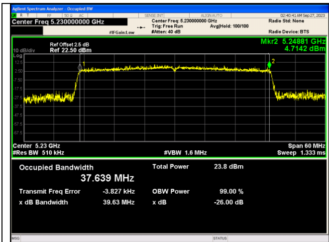
IEEE 802.11ax_Channel 46_40MHz_Antenna 2_RU&Index 484RU65
