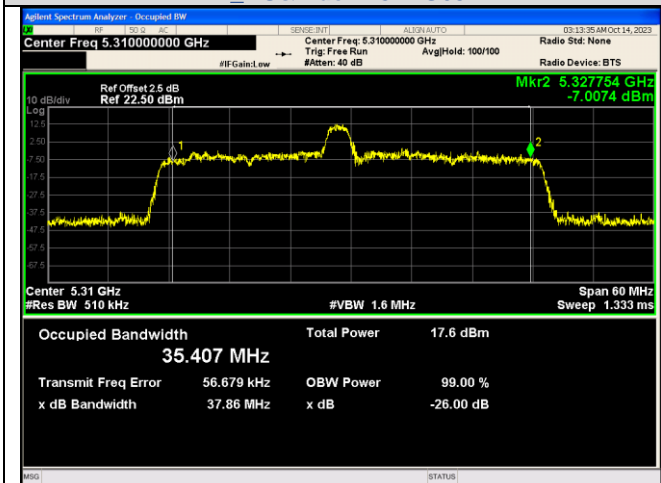
IEEE 802.11ax_Channel 62_40MHz_Antenna 2_RU&Index 26RU8
