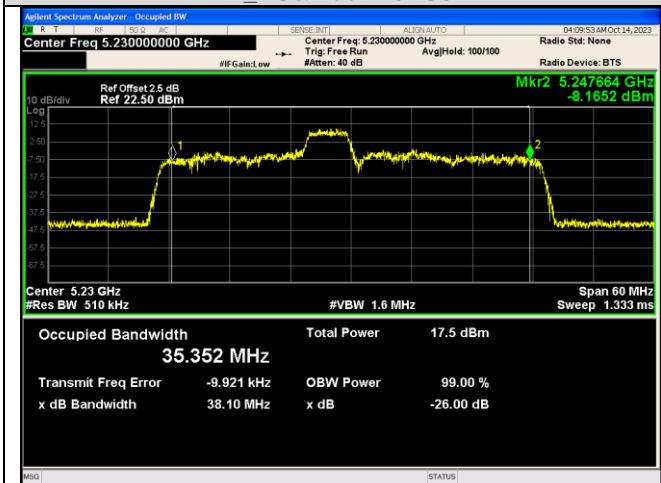
IEEE 802.11ax_Channel 46_40MHz_Antenna 2_RU&Index 52RU40
