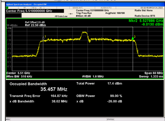
IEEE 802.11ax_Channel 102_40MHz_Antenna 2_RU&Index 26RU8
