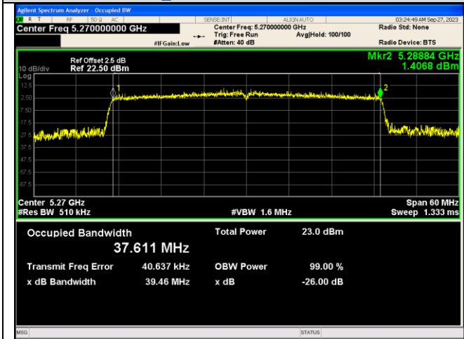
IEEE 802.11ax_Channel 54_40MHz_Antenna 2_RU&Index 484RU65
