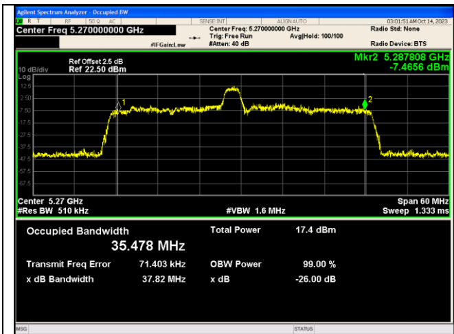
IEEE 802.11ax_Channel 54_40MHz_Antenna 2 RU&Index 26RU8
