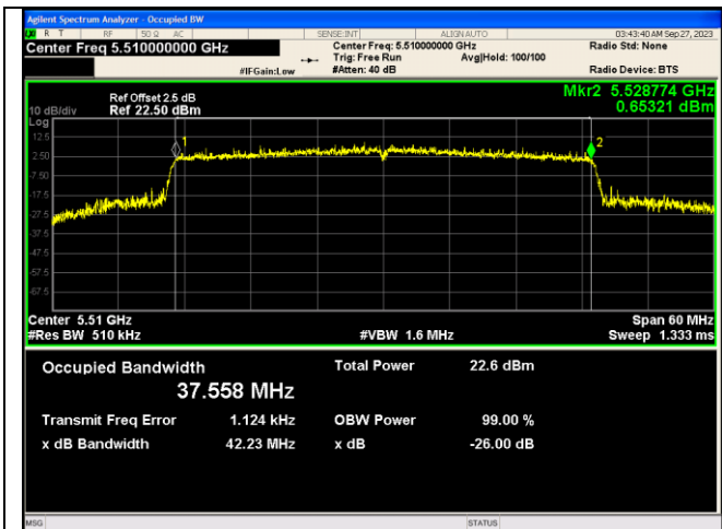
IEEE 802.11ax_Channel 102_40MHz_Antenna 2_RU&Index 484RU65
