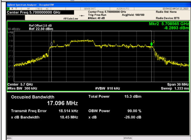
IEEE 802.11ax_Channel 140_20MHz_Antenna 2_RU&Index 26RU38
