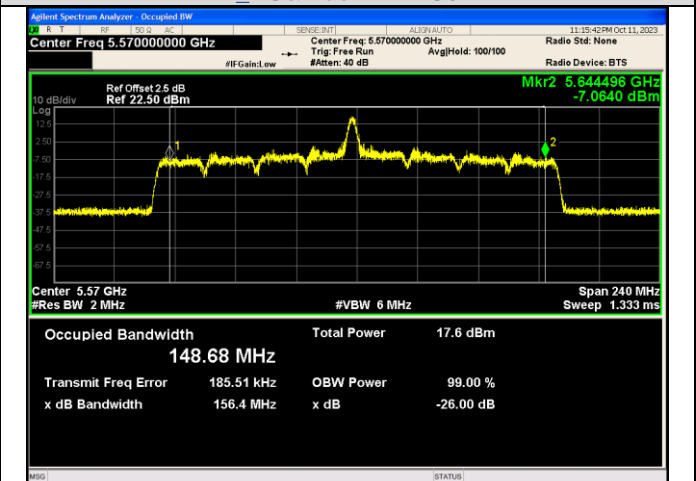
IEEE 802.11ax_Channel 114_160MHz_Antenna 1_RU&Index 26RU36
