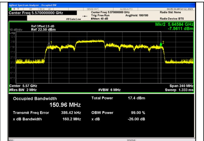
IEEE 802.11ax_Channel 114_160MHz_Antenna 1_RU&Index 484RU66
