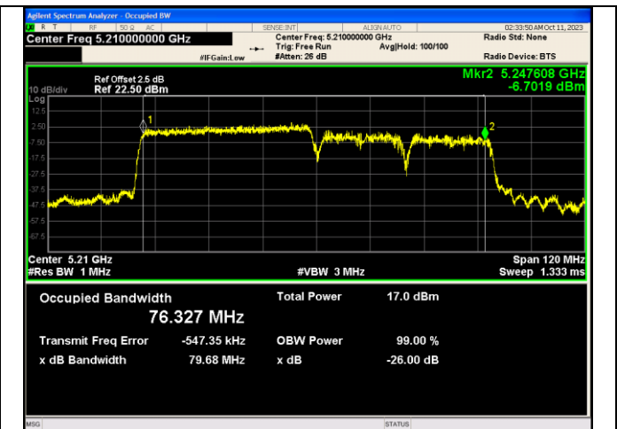
IEEE 802.11ax_Channel 42_80MHz_Antenna 1_RU&Index 484RU65
