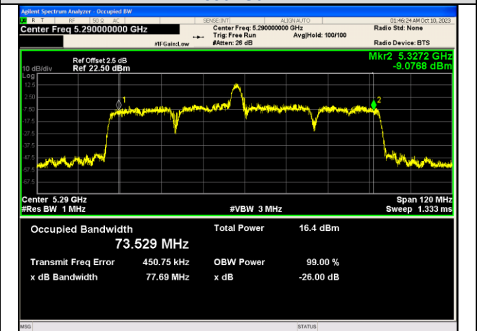
IEEE 802.11ax_Channel 58_80MHz_Antenna 1_RU&Index 26RU17
