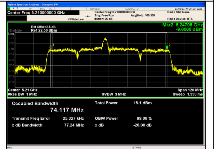
IEEE 802.11ax_Channel 42_80MHz_Antenna 1_RU&Index 26RU17
