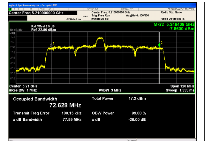
IEEE 802.11ax_Channel 42_80MHz_Antenna 1_RU&Index 52RU44
