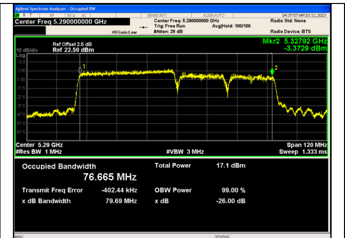
IEEE 802.11ax_Channel 58_80MHz_Antenna 1_RU&Index 484RU65
