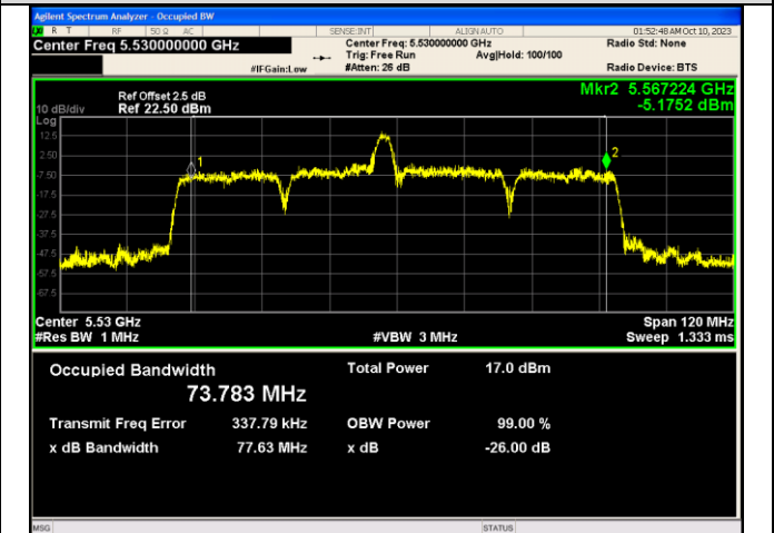
IEEE 802.11ax_Channel 106_80MHz_Antenna 1_RU&Index 26RU17
