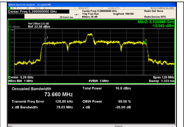
IEEE 802.11ax_Channel 58_80MHz_Antenna 1_RU&Index 52RU44
