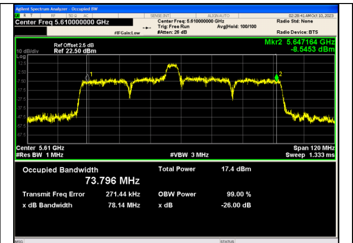
IEEE 802.11ax_Channel 122_80MHz_Antenna 1_RU&Index 52RU44
