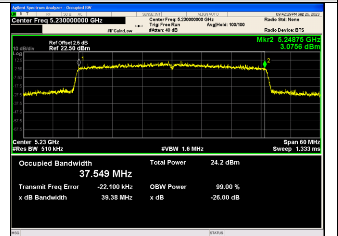
IEEE 802.11ax_Channel 46_40MHz_Antenna 1_RU&Index 484RU65
