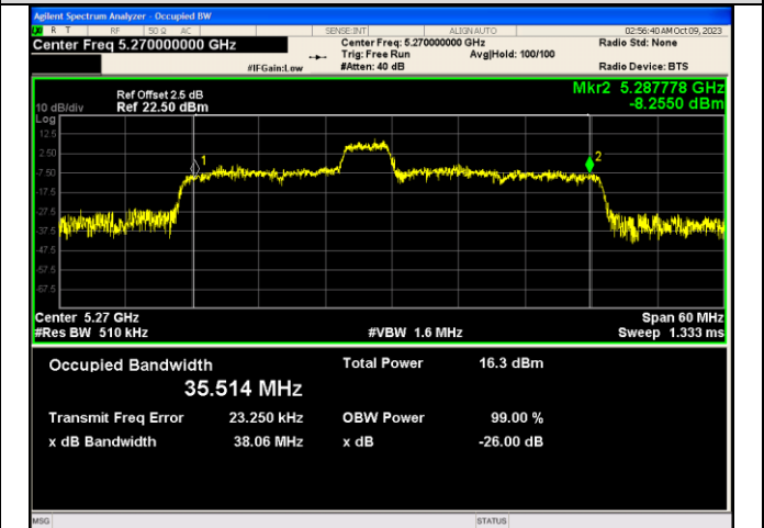
IEEE 802.11ax_Channel 54_40MHz_Antenna 1_RU&Index 52RU40
