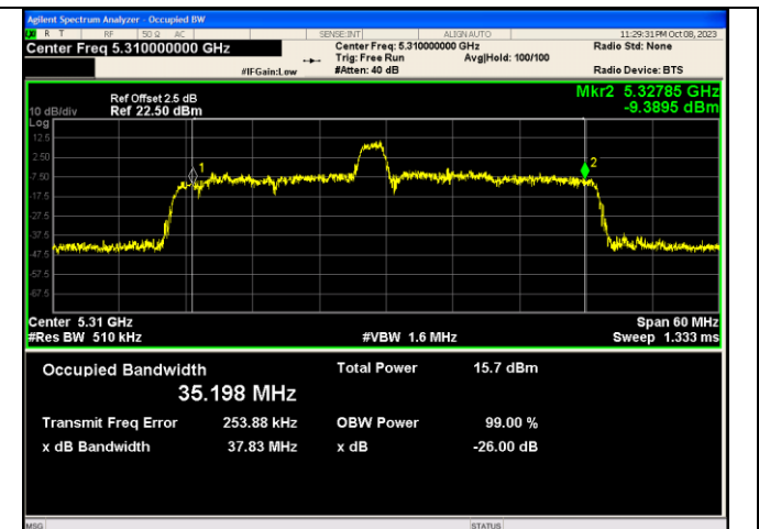
IEEE 802.11ax_Channel 62_40MHz_Antenna 1_RU&Index 26RU8
