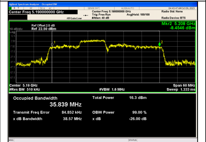
IEEE 802.11ax_Channel 38_40MHz_Antenna 1_RU&Index 106RU54
