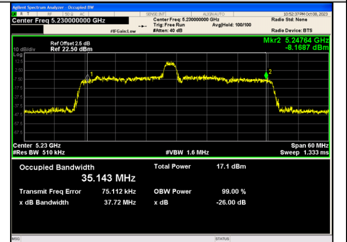
IEEE 802.11ax_Channel 46_40MHz_Antenna 1_RU&Index 26RU8
