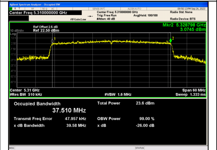
IEEE 802.11ax_Channel 62_40MHz_Antenna 1_RU&Index 484RU65
