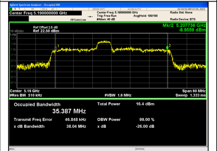
IEEE 802.11ax_Channel 38_40MHz_Antenna 1_RU&Index 52RU40
