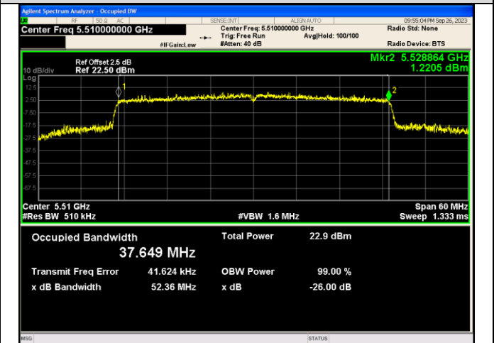
IEEE 802.11ax_Channel 102_40MHz_Antenna 1_RU&Index 484RU65
