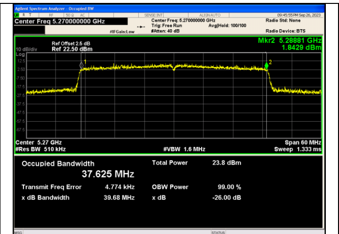
IEEE 802.11ax_Channel 54_40MHz_Antenna 1_RU&Index 484RU65
