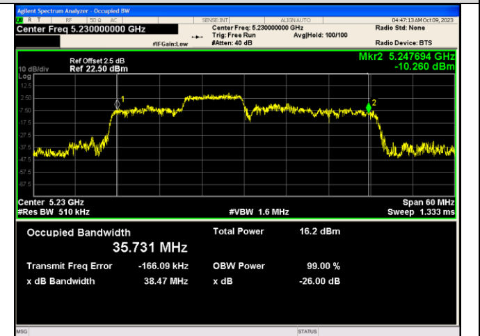
IEEE 802.11ax_Channel 46_40MHz_Antenna 1_RU&Index 106RU54
