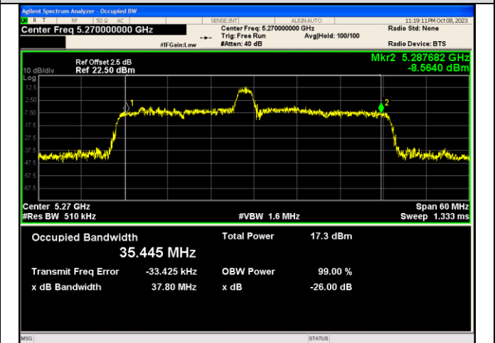
IEEE 802.11ax_Channel 54_40MHz_Antenna 1_RU&Index 26RU8
