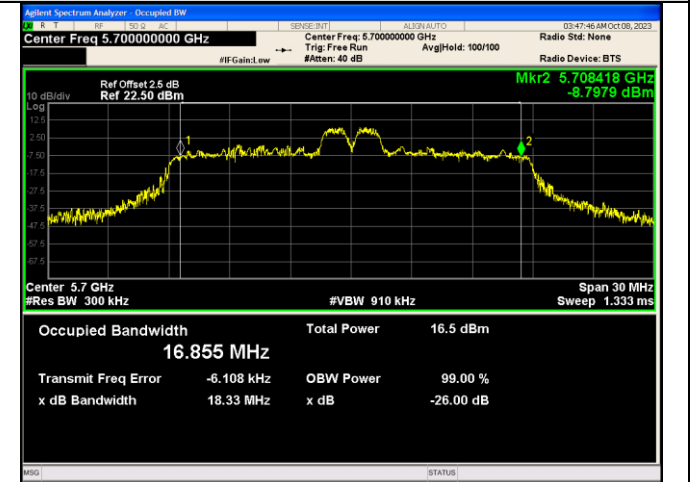
IEEE 802.11ax_Channel 140_20MHz_Antenna 1_RU&Index 26RU4
