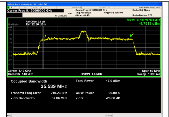
IEEE 802.11ax_Channel 38_40MHz_Antenna 1_RU&Index 26RU8
