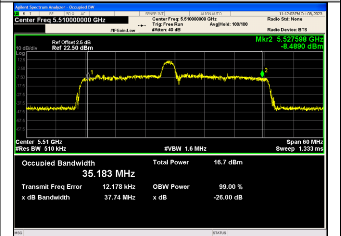
IEEE 802.11ax_Channel 102_40MHz_Antenna 1_RU&Index 26RU8
