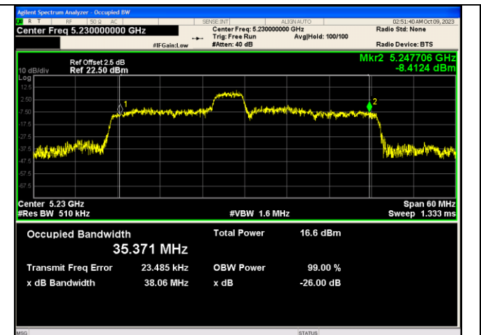
IEEE 802.11ax_Channel 46_40MHz_Antenna 1_RU&Index 52RU40
