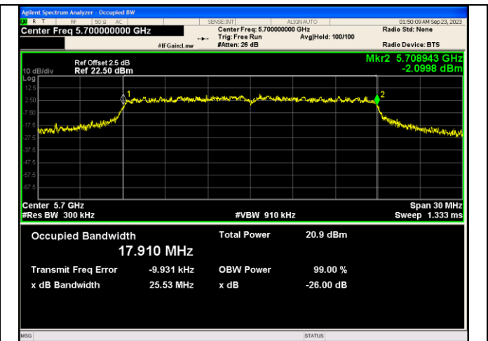
IEEE 802.11ac Channel 140 20MHz Antenna 1
