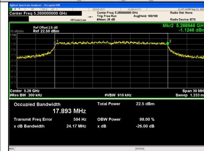
IEEE 802.11ac Channel 52 20MHz Antenna 1
