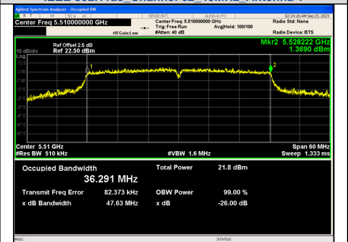
IEEE 802.11ac Channel 102 40MHz Antenna 1
