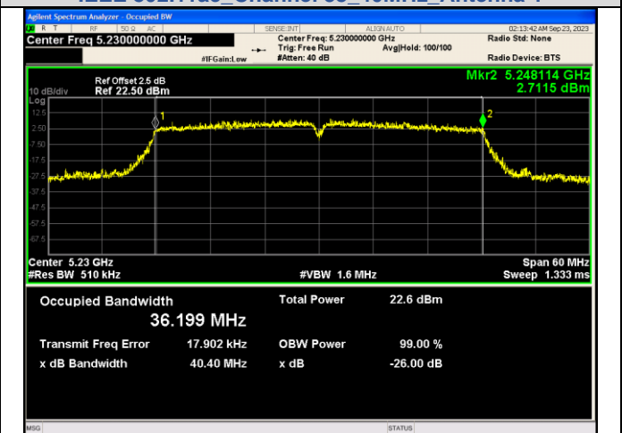
IEEE 802.11ac Channel 46 40MHz Antenna 1
