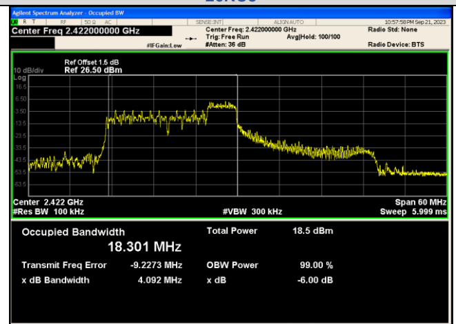
IEEE 802.11ax_Channel 3_40MHz_Antenna 1_RU&Index 52RU40
