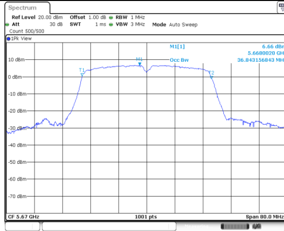
11N40SISO_Ant1_5670
