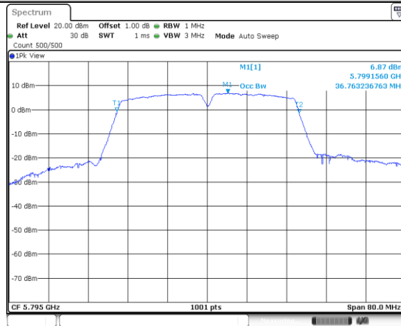
11AC40SISO_Ant1_5795
