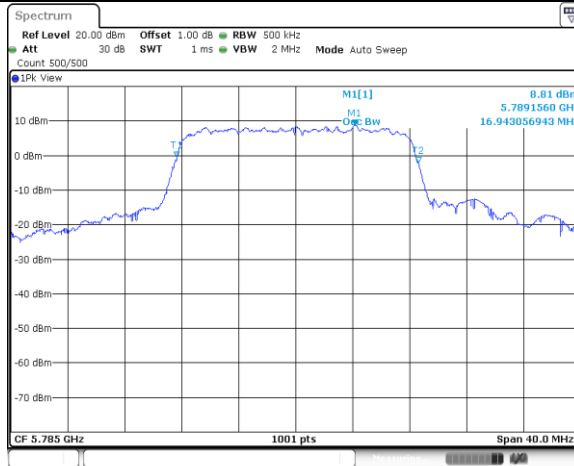
11A_Ant1_5785
