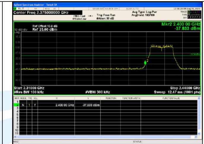
Out Of Band Emission IEEE 802.11g_Channel 1_20MHz_Antenna 0
