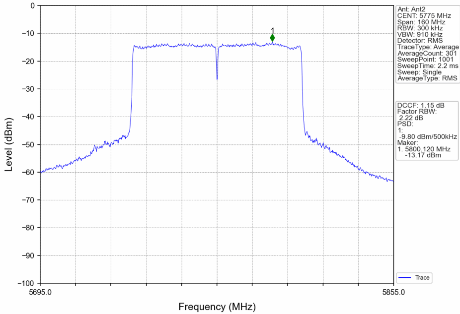
802.11ac(VHT80)_MCH_5775MHz_MIMO_NTNV
