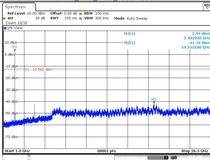
3DH5_Ant1_2402_1000~26500
