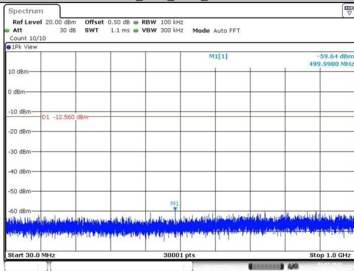
3DH5_Ant1_2402_30~1000
