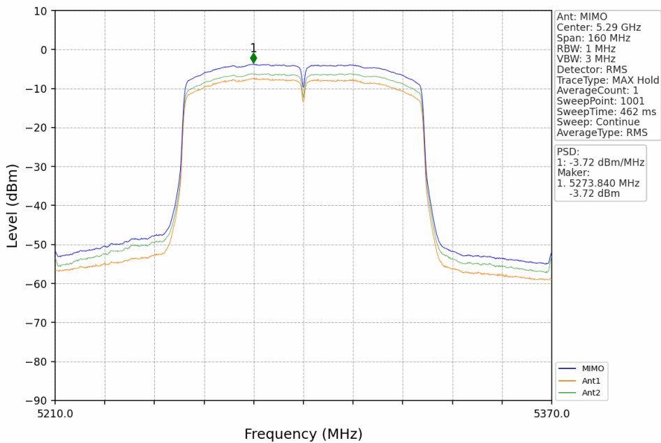
802.11ac(VHT80)_MCH_5290MHz_MIMO_NTNV
