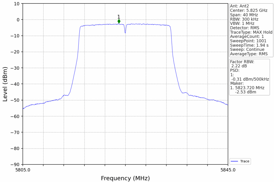
802.11ac(VHT20)_HCH_5825MHz_MIMO_NTNV
