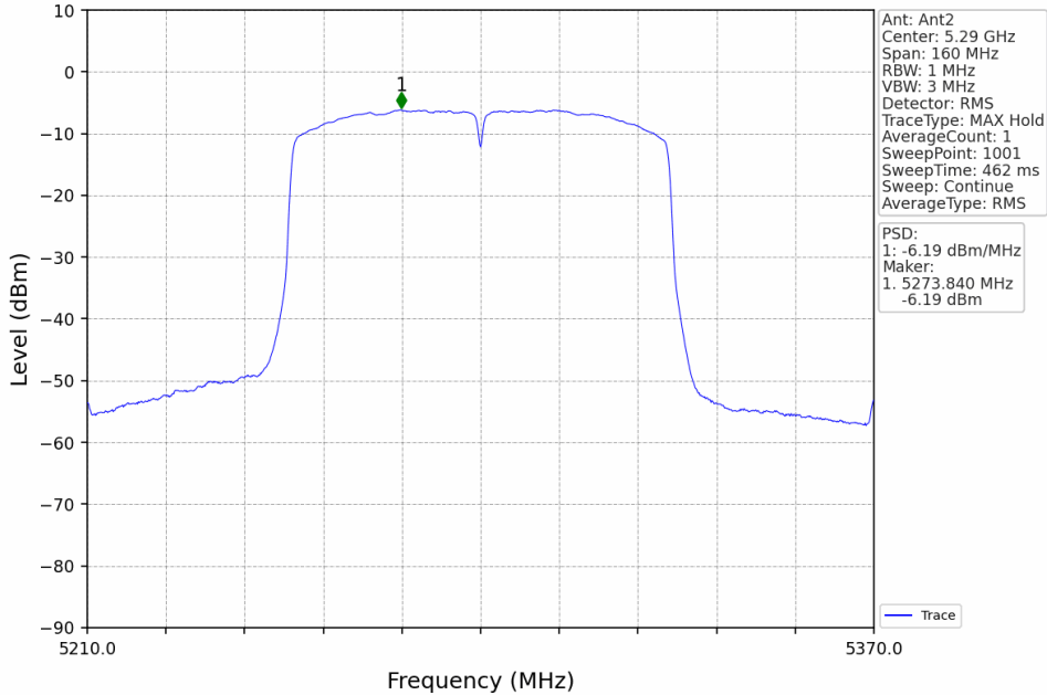
802.11ac(VHT80)_MCH_5290MHz_MIMO_NTNV
