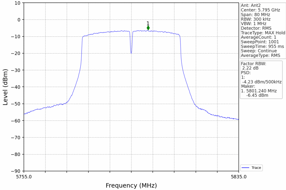
802.11ac(VHT40)_HCH_5795MHz_MIMO_NTNV
