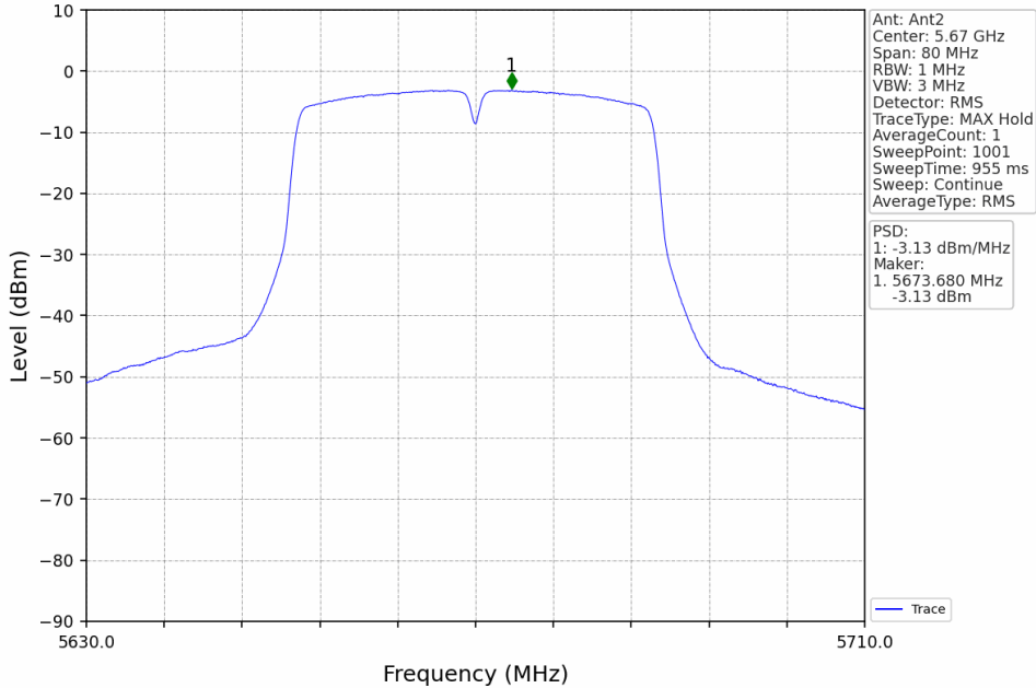
802.11ac(VHT40)_HCH_5670MHz_MIMO_NTNV
