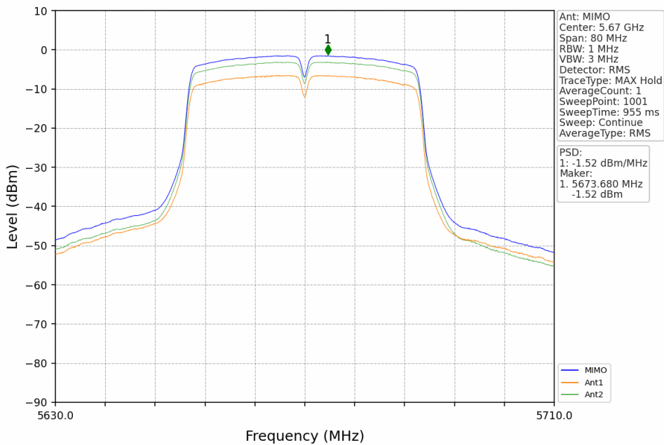
802.11ac(VHT40)_HCH_5670MHz_MIMO_NTNV
