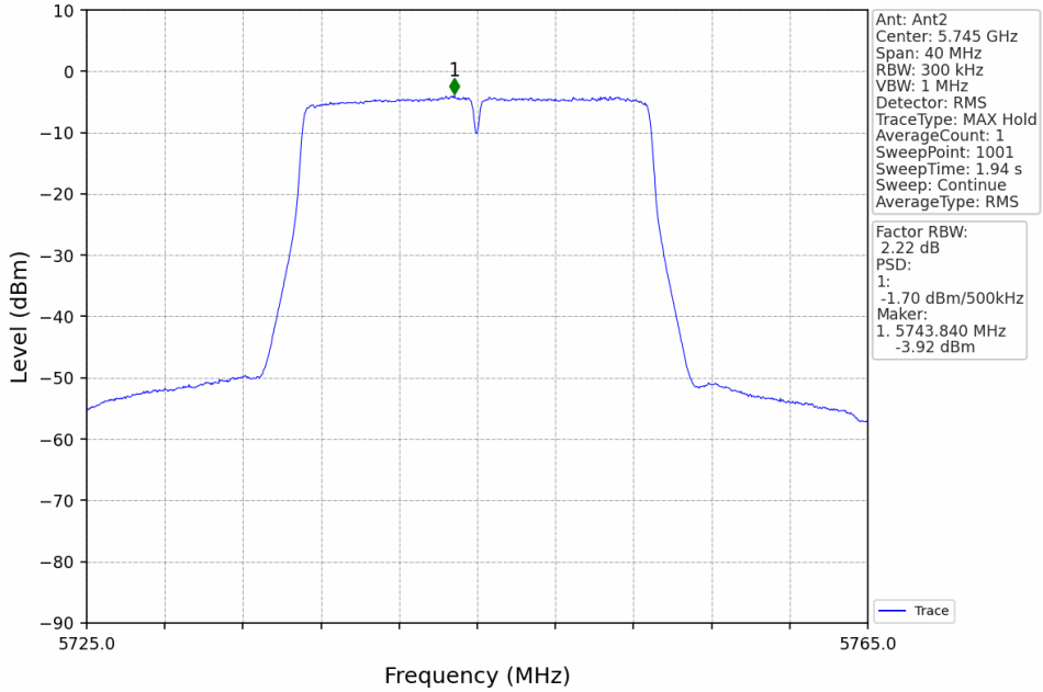
802.11ac(VHT20)_LCH_5745MHz_MIMO_NTNV
