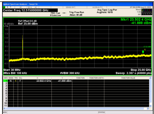
Spurious Emission IEEE 802.11ax_Channel 3_40MHz_Antenna 1_RU&Index 26RU0
