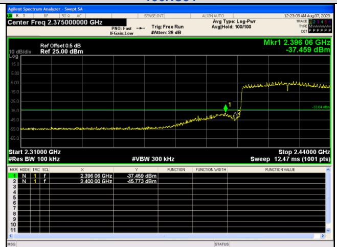
Out Of Band Emission IEEE 802.11ax_Channel 3_40MHz_Antenna 0_RU&Index 484RU65
