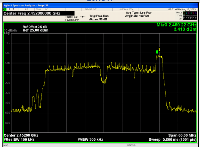
In-Band Reference Level IEEE 802.11ax_Channel 9_40MHz_Antenna 1_RU&Index 26RU17
