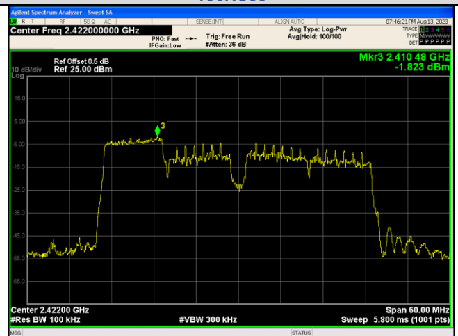
In-Band Reference Level IEEE 802.11ax_Channel 3_40MHz_Antenna 1_RU&Index 106RU53
