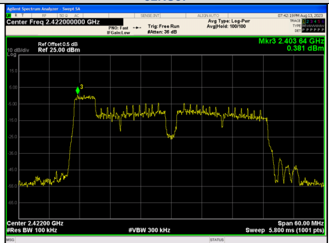
In-Band Reference Level IEEE 802.11ax_Channel 3_40MHz_Antenna 1_RU&Index 52RU37
