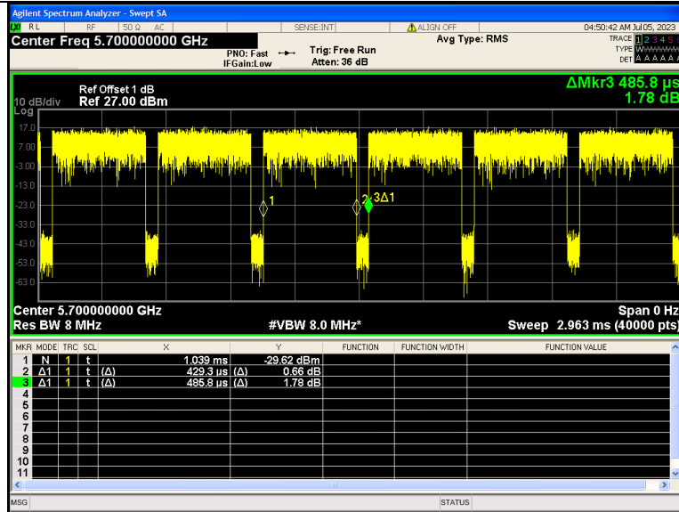
IEEE 802.11ax 20MHz Channel 140
