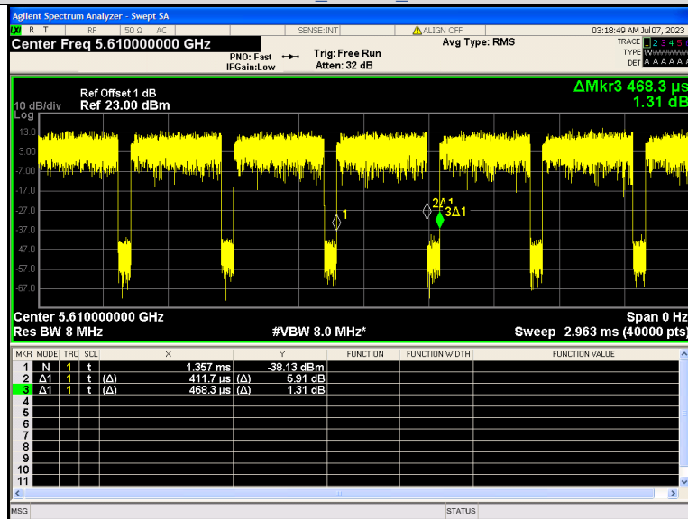
IEEE 802.11ax 80MHz Channel 122
