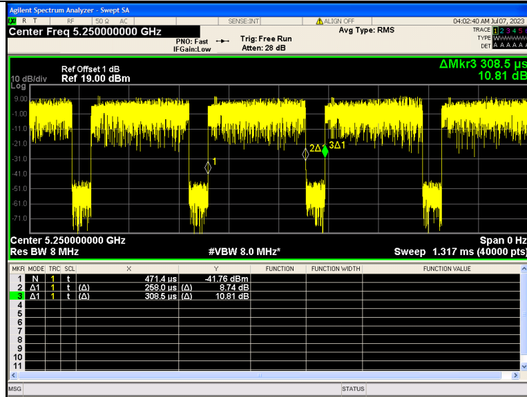
IEEE 802.11ax 160MHz Channel 50
