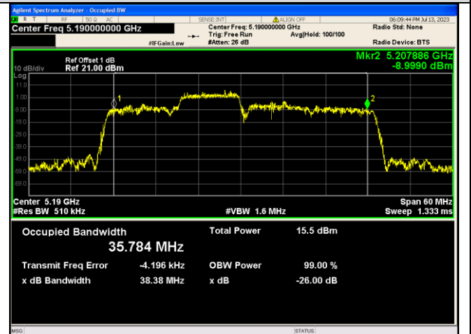
IEEE 802.11ax_Channel 38_40MHz_Antenna 1_RU&Index 106RU54
