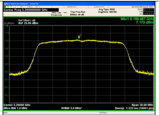
IEEE 802.11n Channel 40 20MHz Antenna 3
