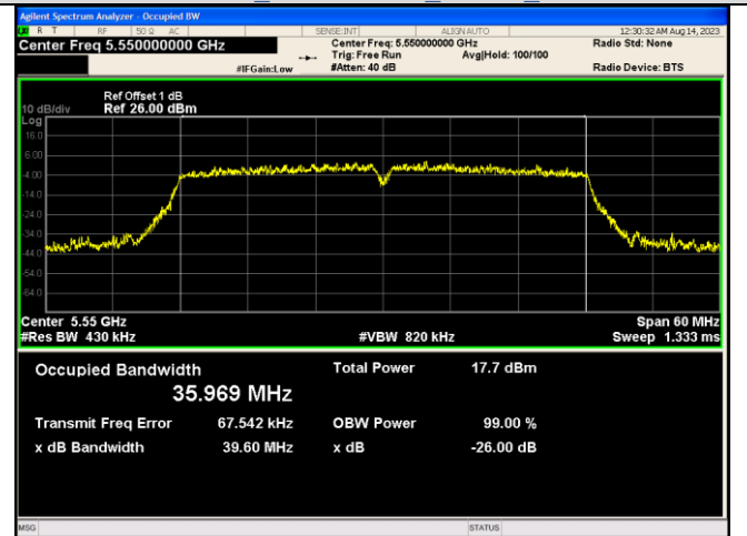
IEEE 802.11ac Channel 110 40MHz Antenna 3
