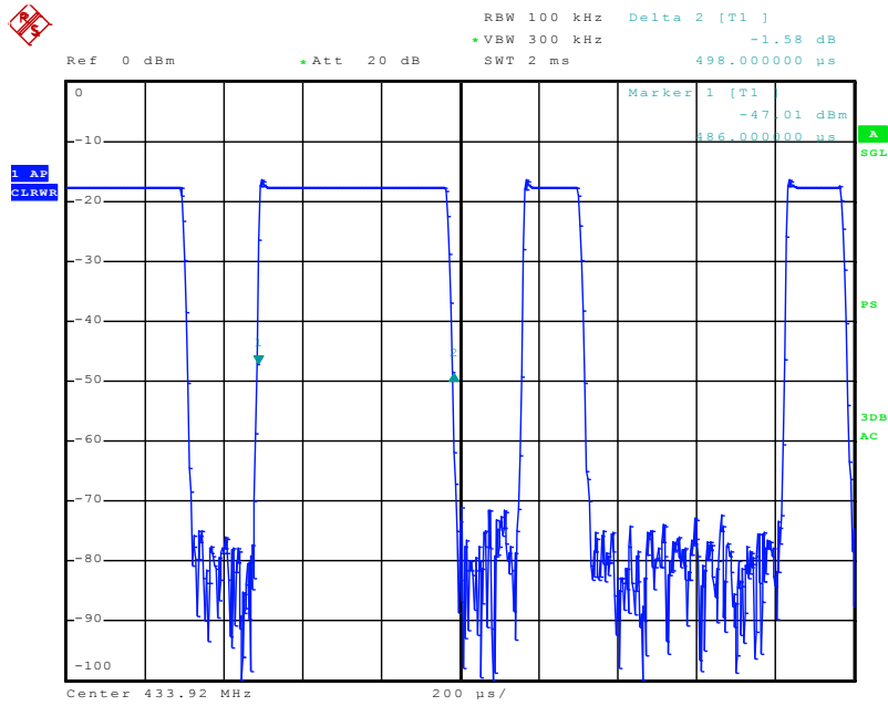
Dwell time of one pulse
