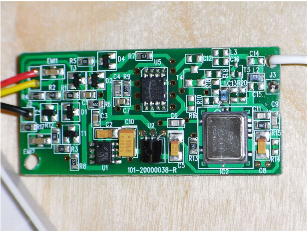
B&S Transmitter PCB including Power latch, Voltage regulator, CPU.
