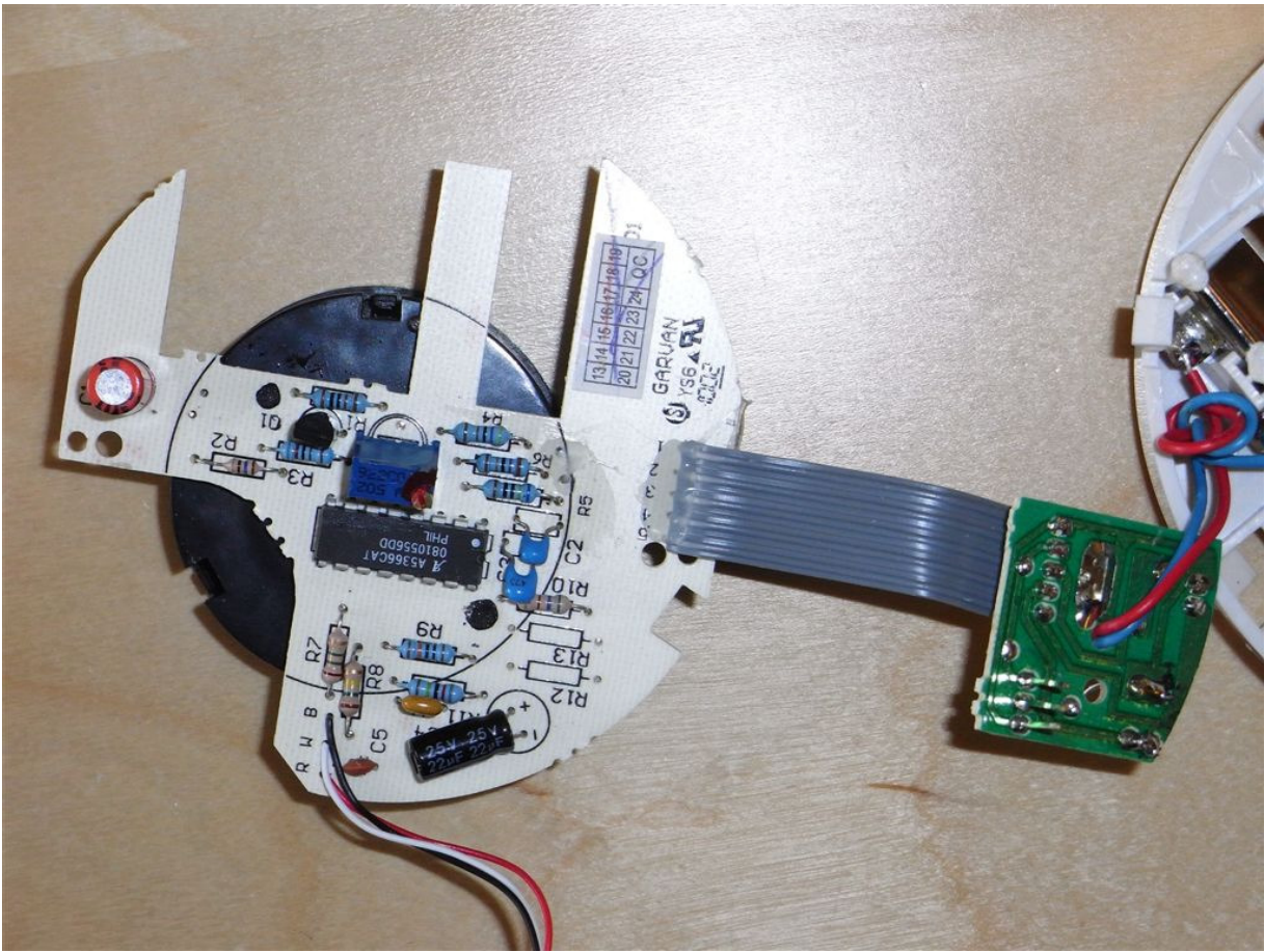
Main Smoke Detector PCB and Connector board for Transmitter.
