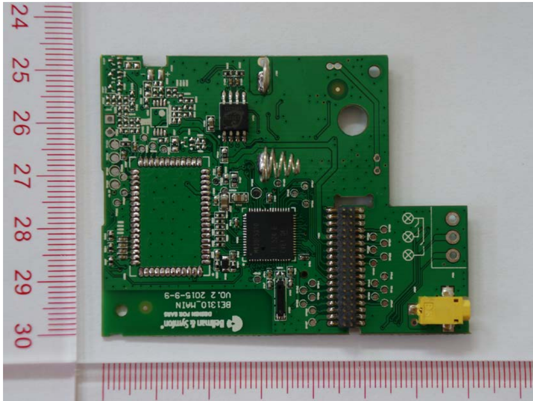
FIGURE 5 VISIT SMART HUB (M/N: BE1310) MAIN BOARD #1 (FRONT VIEW WITHOUT BT MODULE)
