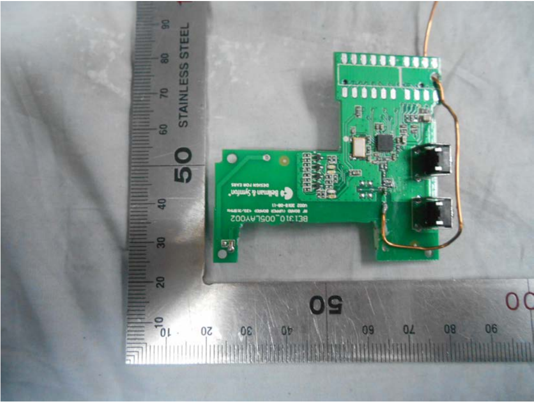
FIGURE 7 VISIT SMART HUB (M/N: BE1310) MAIN BOARD #2 (FRONT VIEW)
