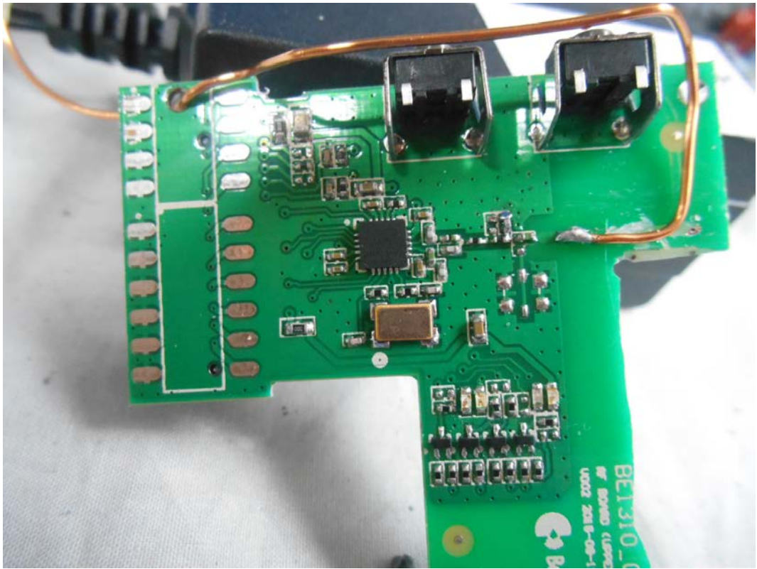
FIGURE 9 VISIT SMART HUB (M/N: BE1310) CHIP AND IC ON MAIN BOARD #2
