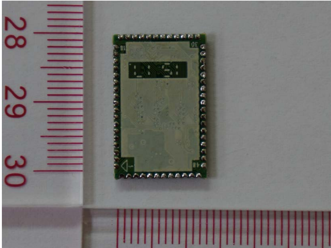
FIGURE 11 VISIT SMART HUB (M/N: BE1310) BT MODULE ON MAIN BOARD #1(BACK VIEW)
