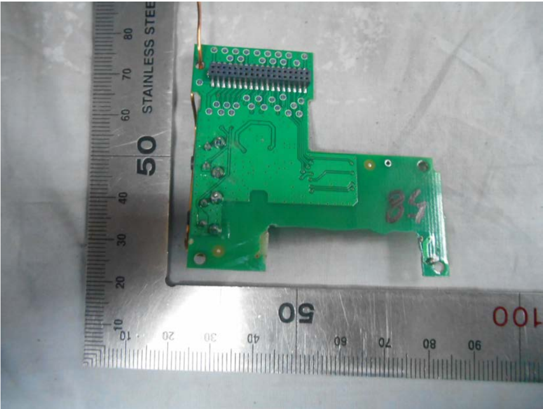
FIGURE 8 VISIT SMART HUB (M/N: BE1310) MAIN BOARD #2 (BACK VIEW)
