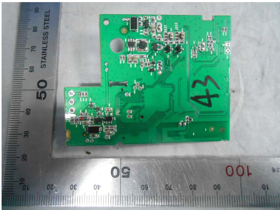
FIGURE 6 VISIT SMART HUB (M/N: BE1310) MAIN BOARD #1 (BACK VIEW)
