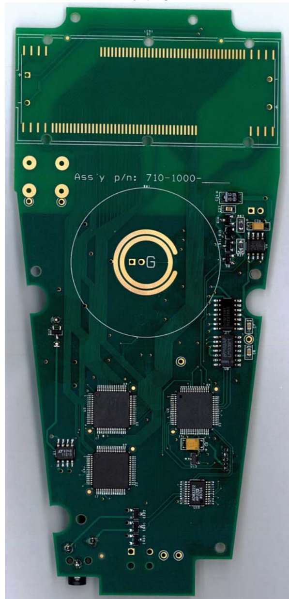
Front PCB
