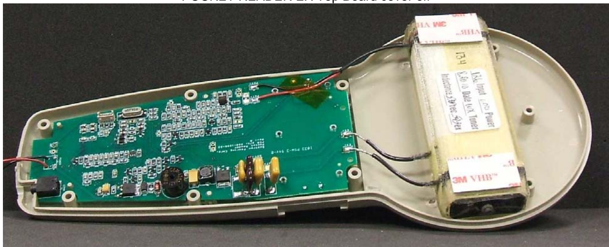
POCKET READER EX Top Board cover off
