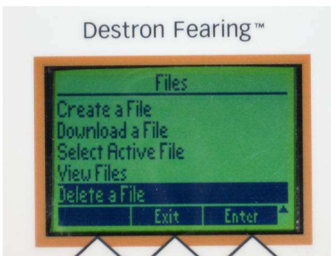
FIG. 48: Files Screen
