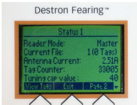
FIG. 13: Status 1 Screen
