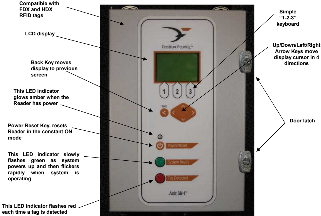
Figure 1: External View of the Model AXIZ SB-1™
