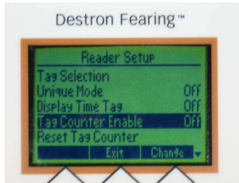
FIG. 68: Reader Setup Screen: Tag Counter Enable OFF
