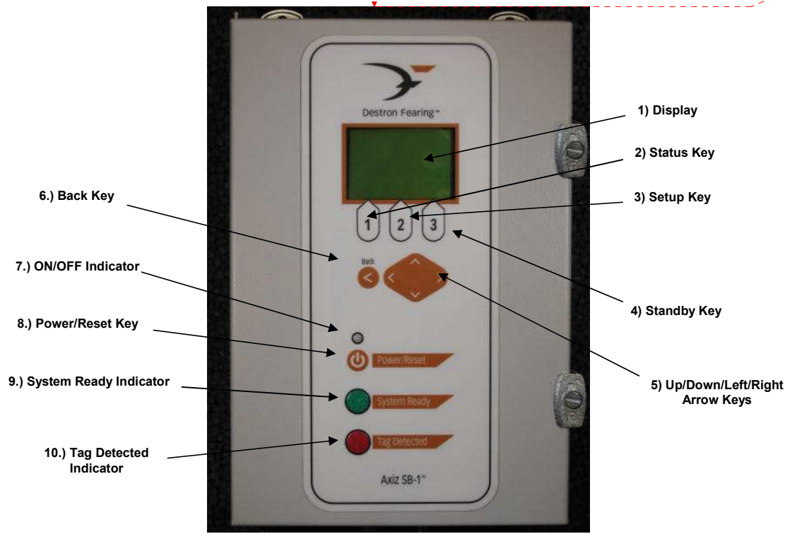
FIG. 2: Control Panel Component Identification
