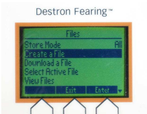
FIG. 31: Files Screen
