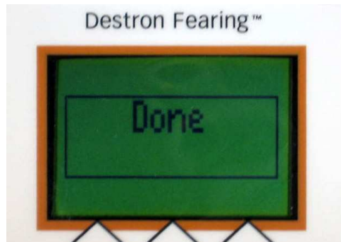
FIG. 38: Done Screen
