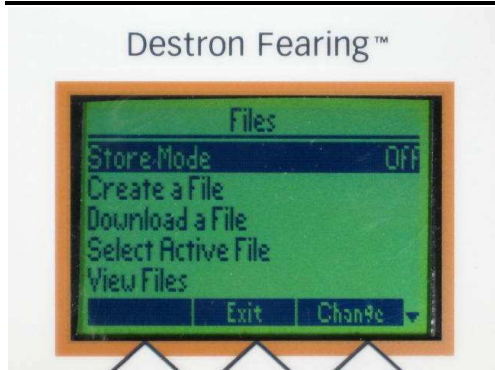
FIG. 26: Files Screen
