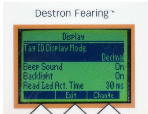
FIG. 96: Display Screen
