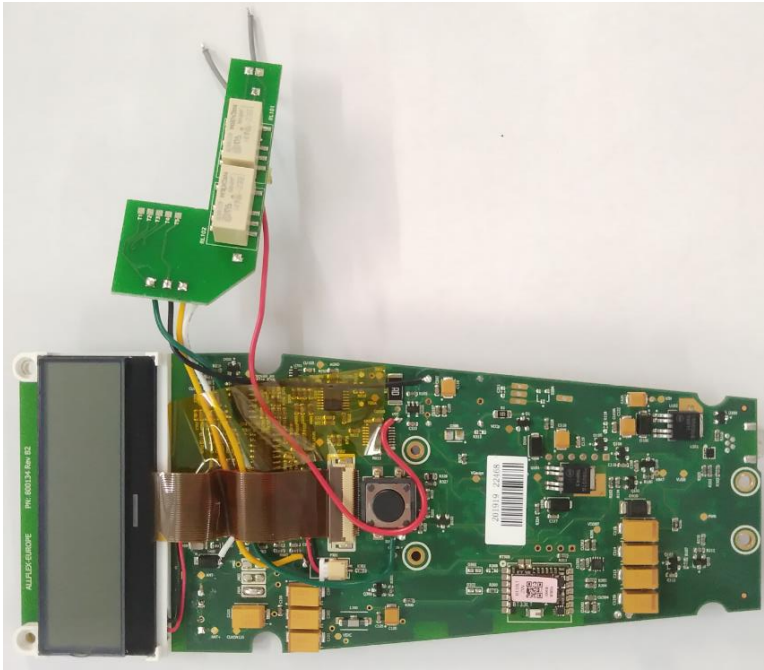
Figure 4: Main PCB with Relay PCB top view.
