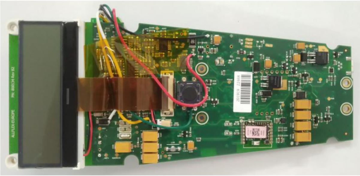
Figure 3: Main PCB top view
