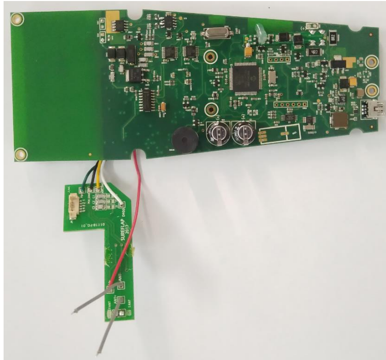
Figure 5: Main PCB bottom view with Relay PCB bottom view.
