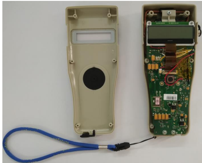
Figure 1: Front cover removed.
