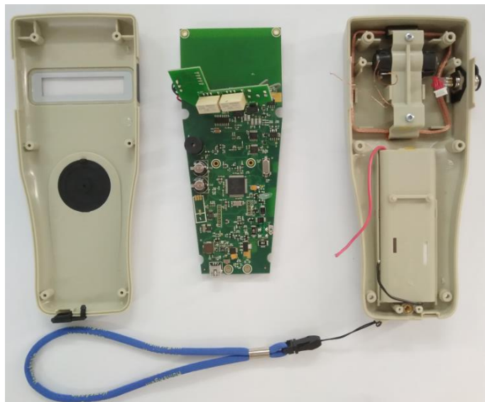
Figure 2: PCB removed.
