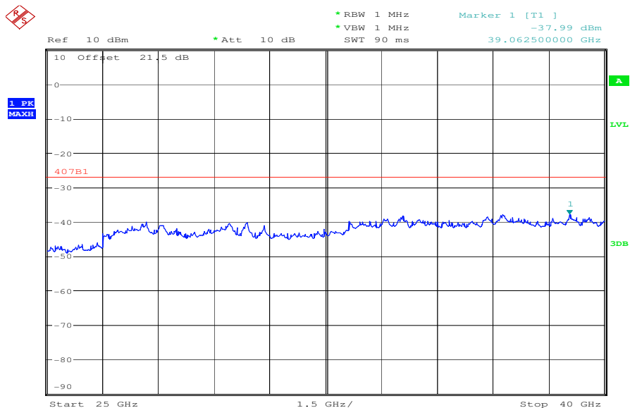
Plot 4: channel 1, 5180 MHz
