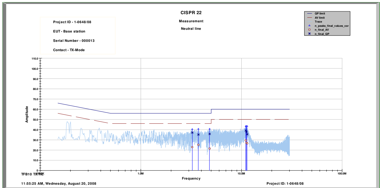
Plot 1: Neutral line TX mode
