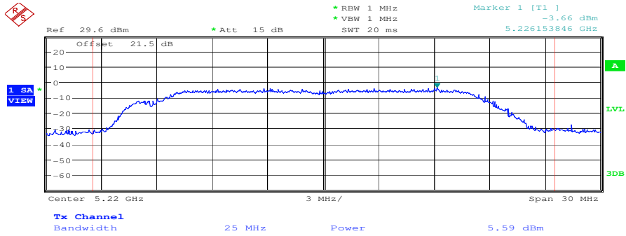
Plot 2: channel 3, 5220 MHz
