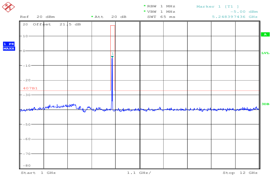
Plot 10: channel 4, 5240 MHz
