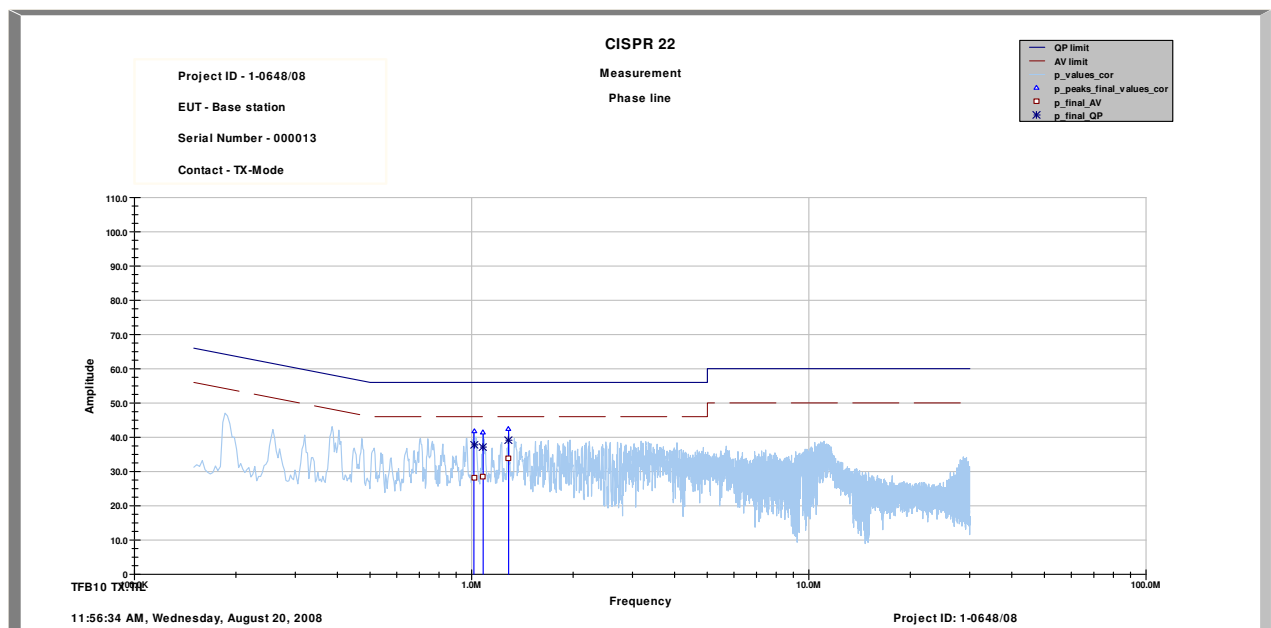
Plot 2: Phase line TX mode
