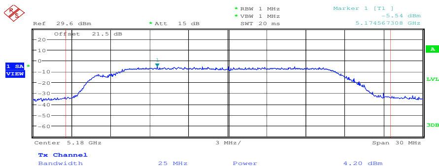
Plot 1: channel 1, 5180 MHz
