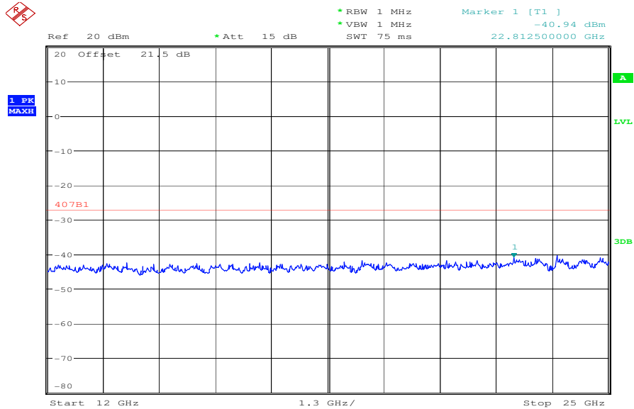
Plot 3: channel 1, 5180 MHz
