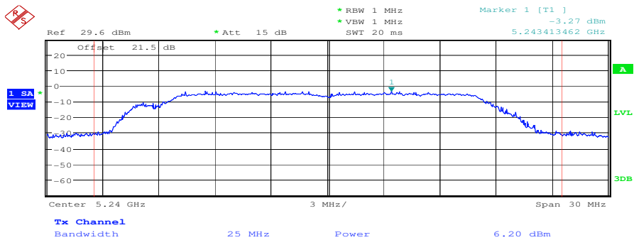
Plot 3: channel 4, 5240 MHz
