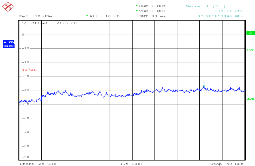
Plot 12: channel 4, 5240 MHz
