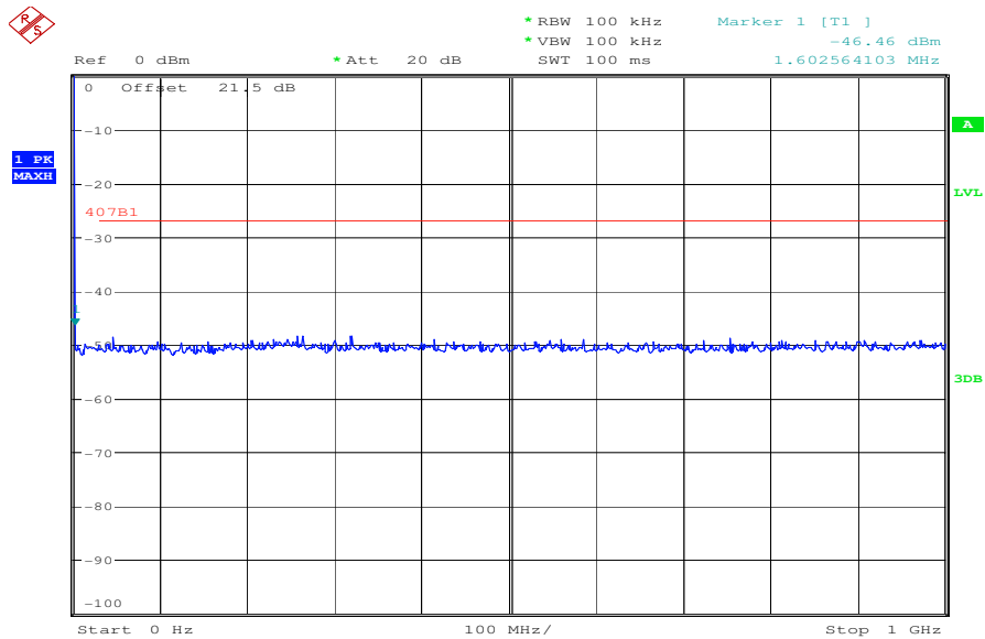
Plot 5: channel 3, 5220 MHz
