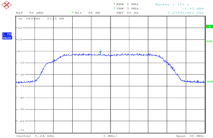
Plot 3: channel 4, 5240 MHz
