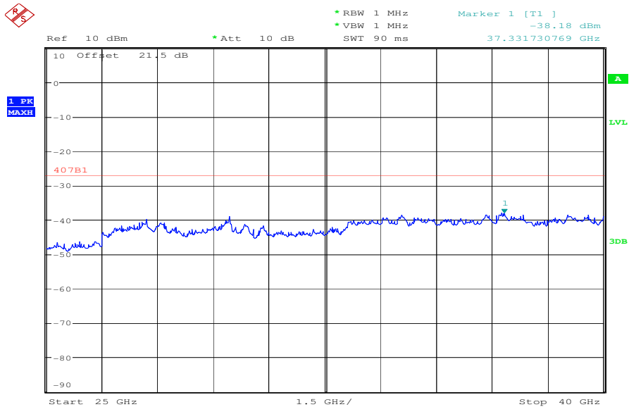
Plot 8: channel 3, 5220 MHz
