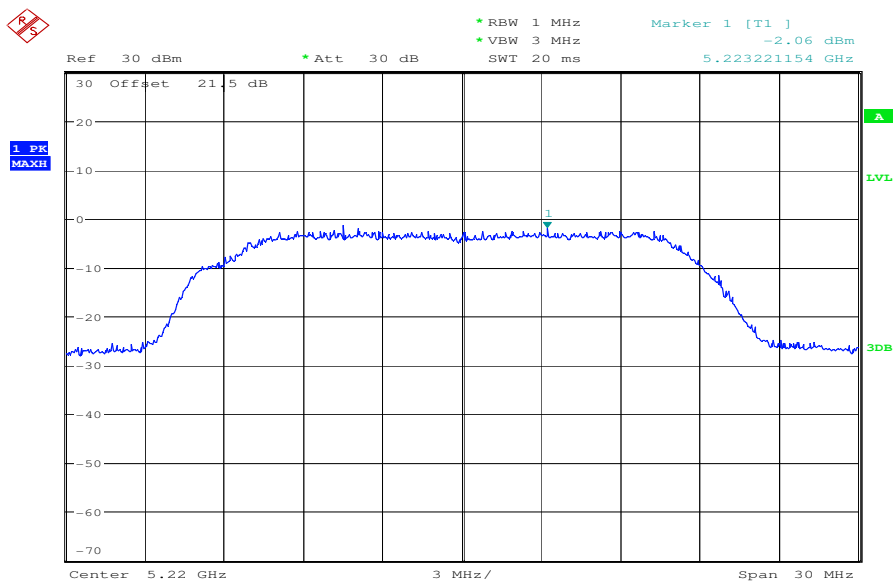
Plot 2: channel 3, 5220 MHz
