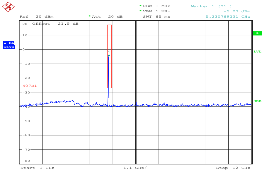
Plot 6: channel 3, 5220 MHz
