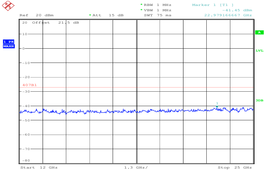
Plot 7: channel 3, 5220 MHz
