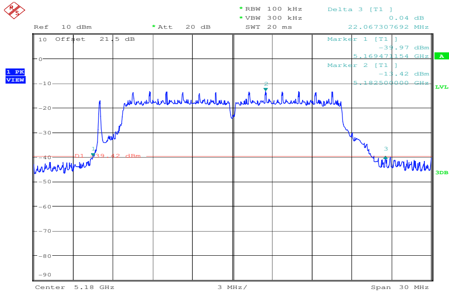
Plot 1: channel 1, 5180 MHz
