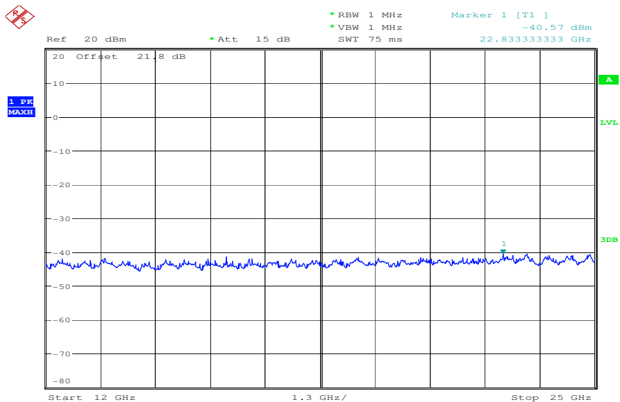
Plot 11: channel 2, 5765 MHz
