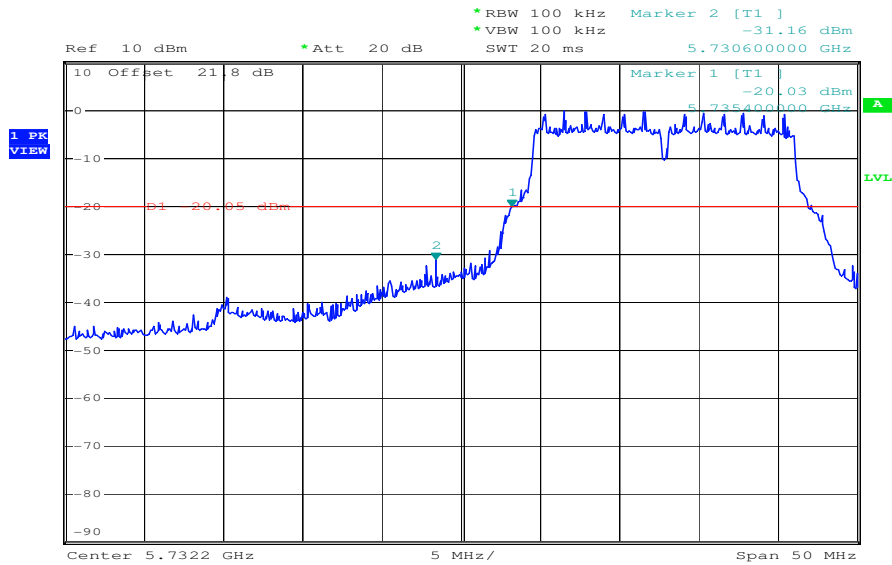
Plot 1: lowest channel, 5745 MHz
