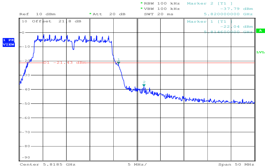
Plot 2: highest channel, 5805 MHz
