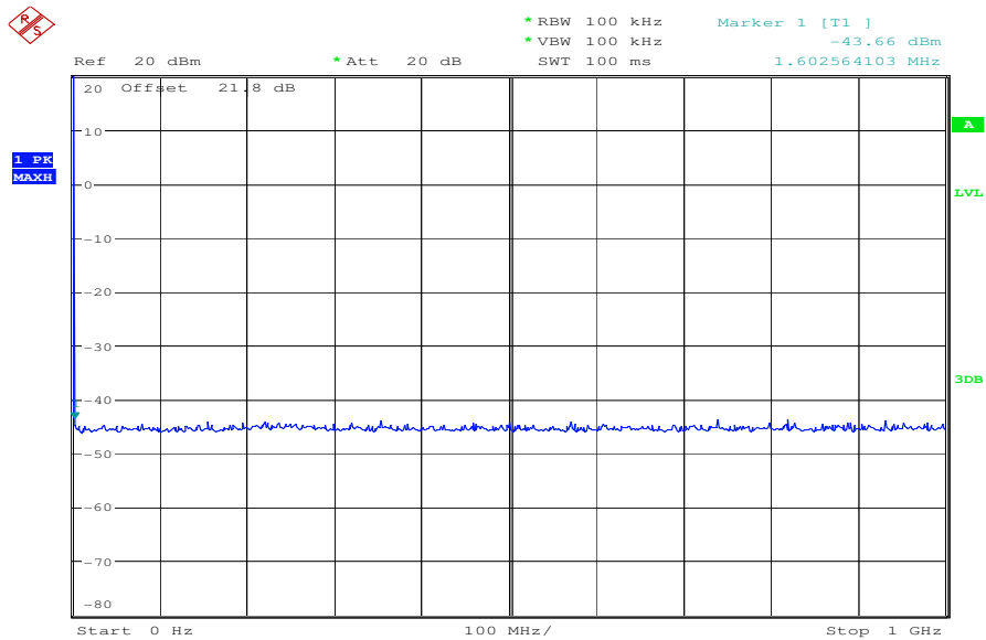
Plot 7: channel 2, 5765 MHz
