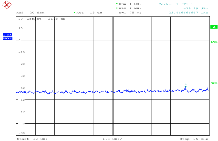
Plot 17: channel 4, 5805 MHz
