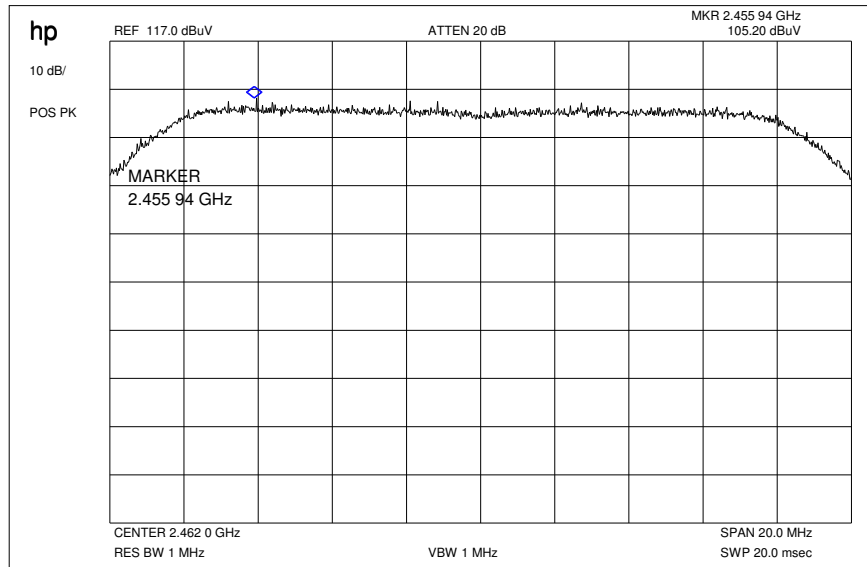
Plot 1: Max field strength in 3m distance (single frequency) peak
