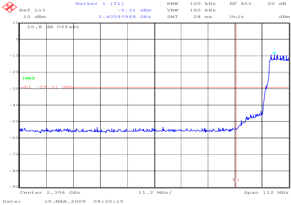
Plot 1: lowest channel
