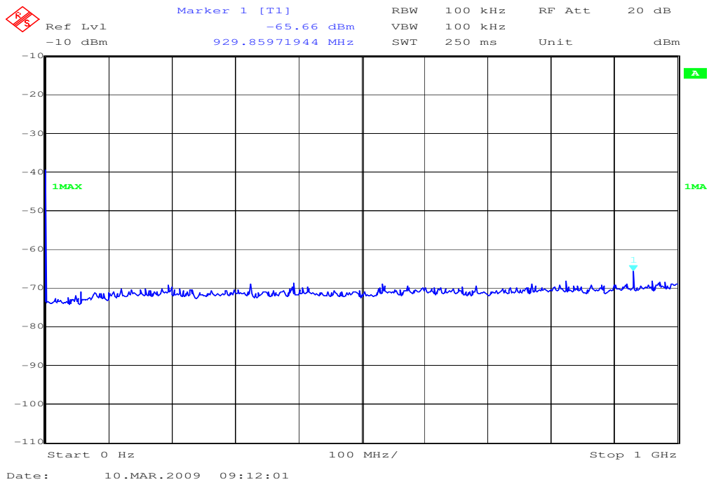
Plot 4: Middle Channel
