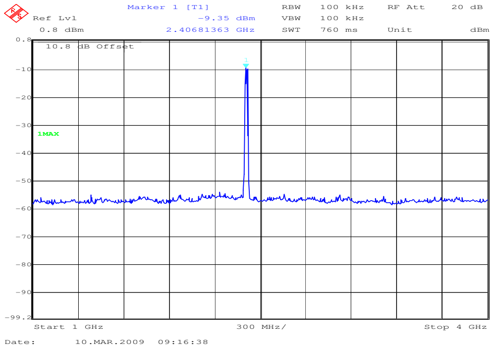
Plot 2: Lowest Channel
