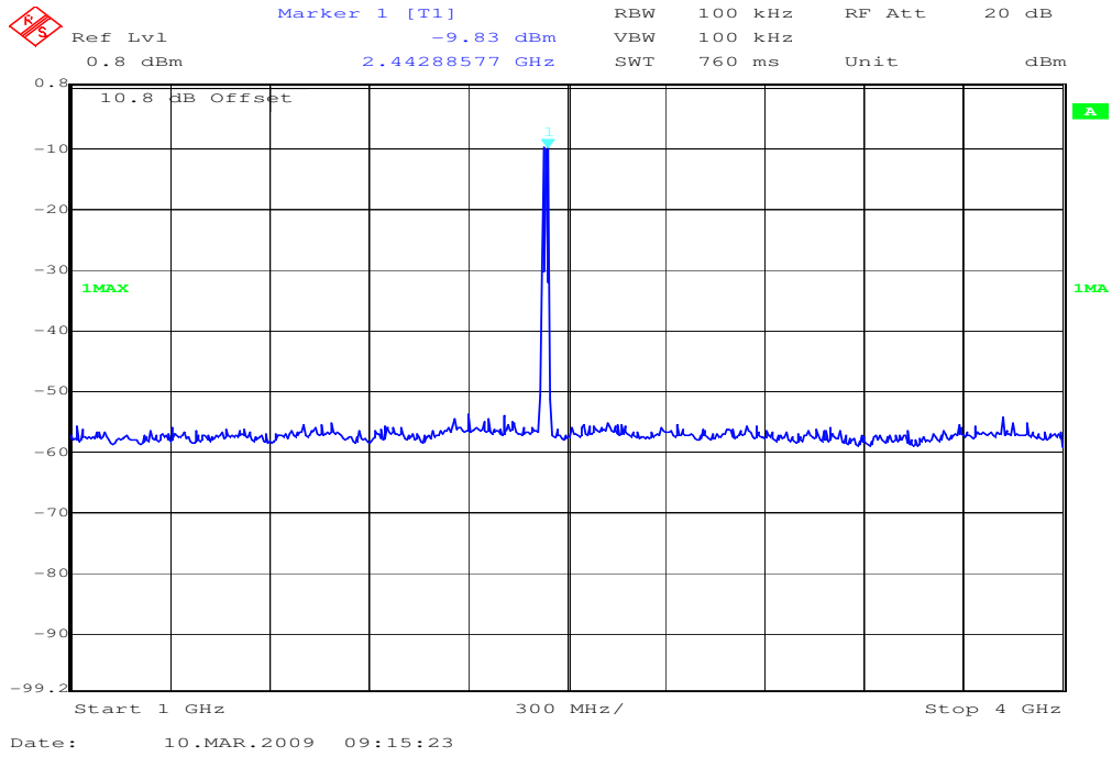
Plot 5: Middle Channel
