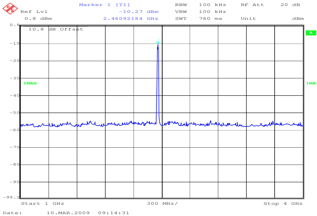
Plot 8: Highest Channel
