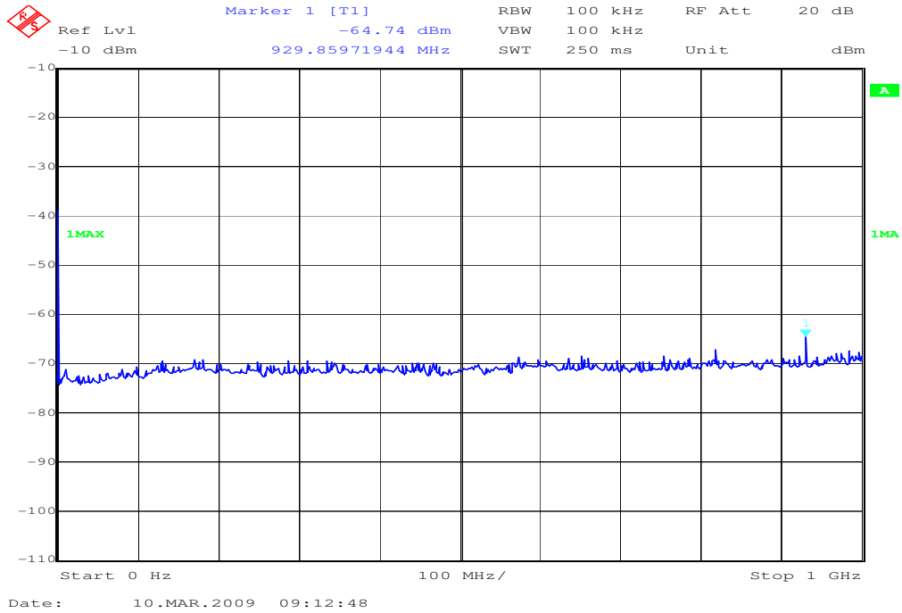
Plot 7: Highest Channel
