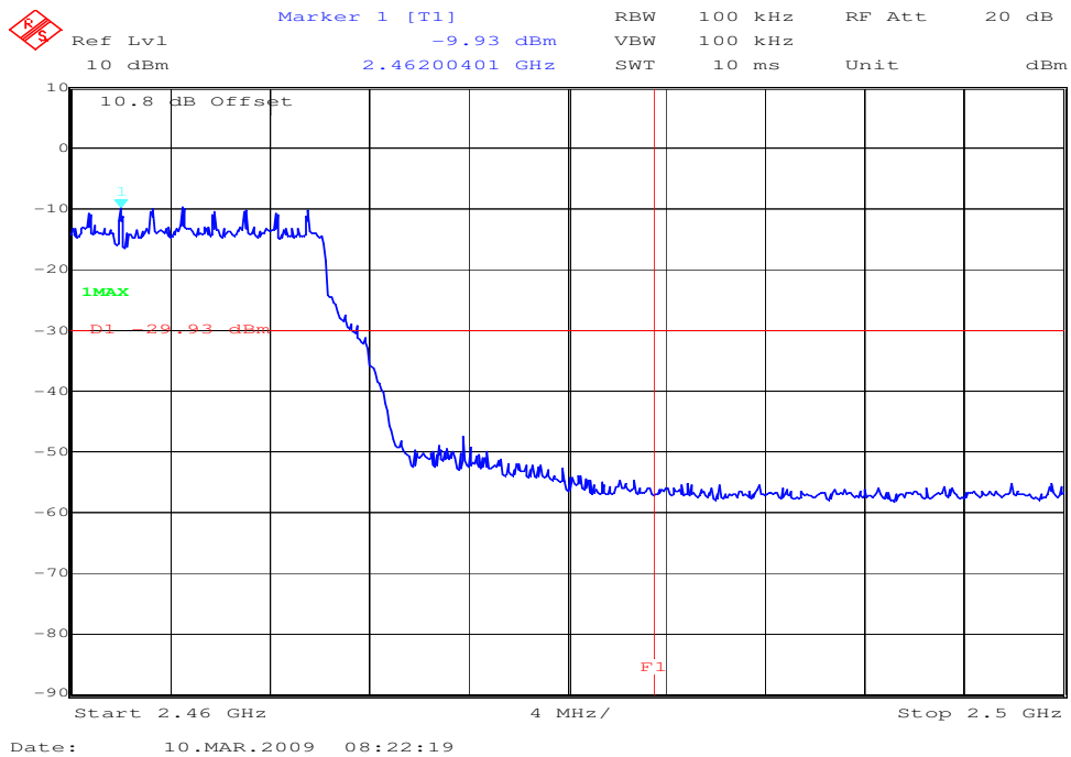
Plot 2: highest channel
