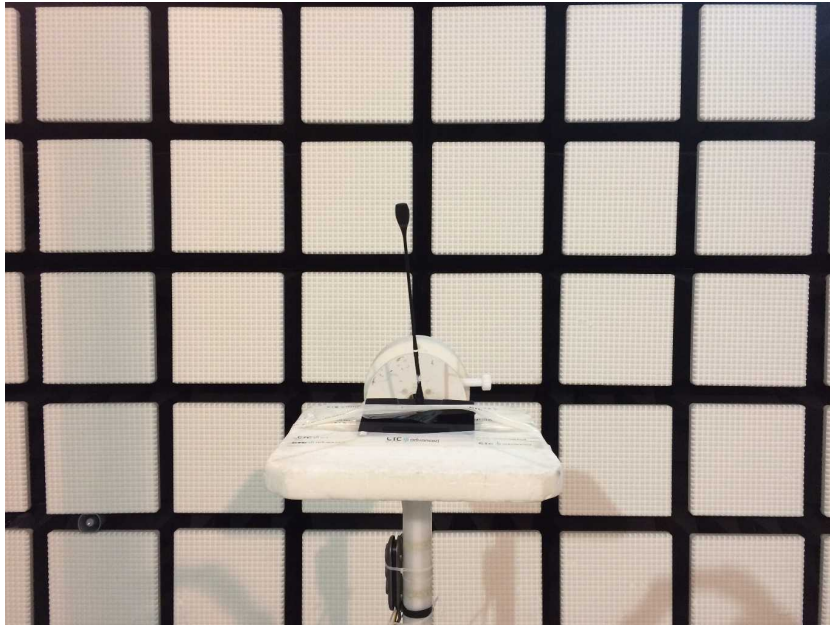
Photo 3 RSE > 1GHz
