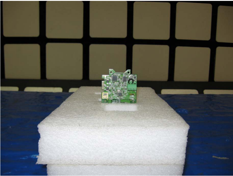
Radiated Emissions – Y Axis
