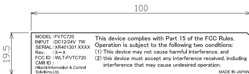
Label detail
