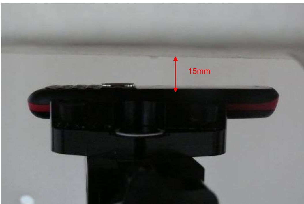
Picture 14: Body, The EUT display towards phantom, the distance from handset to the bottom of the Phantom is 15mm
