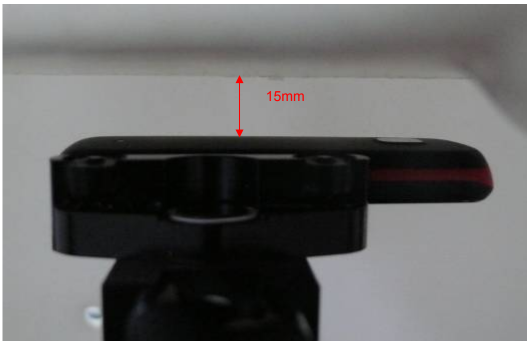
Picture 13: Body, The EUT display towards ground, the distance from handset to the bottom of the Phantom is 15mm
