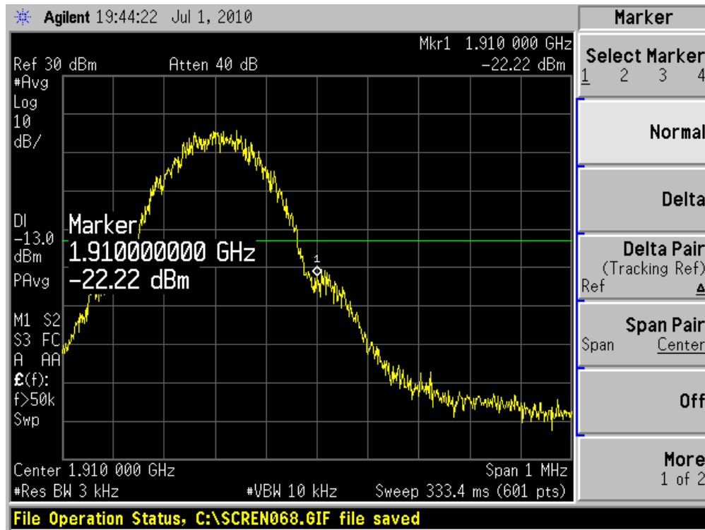
GSM1900 810 Channel
