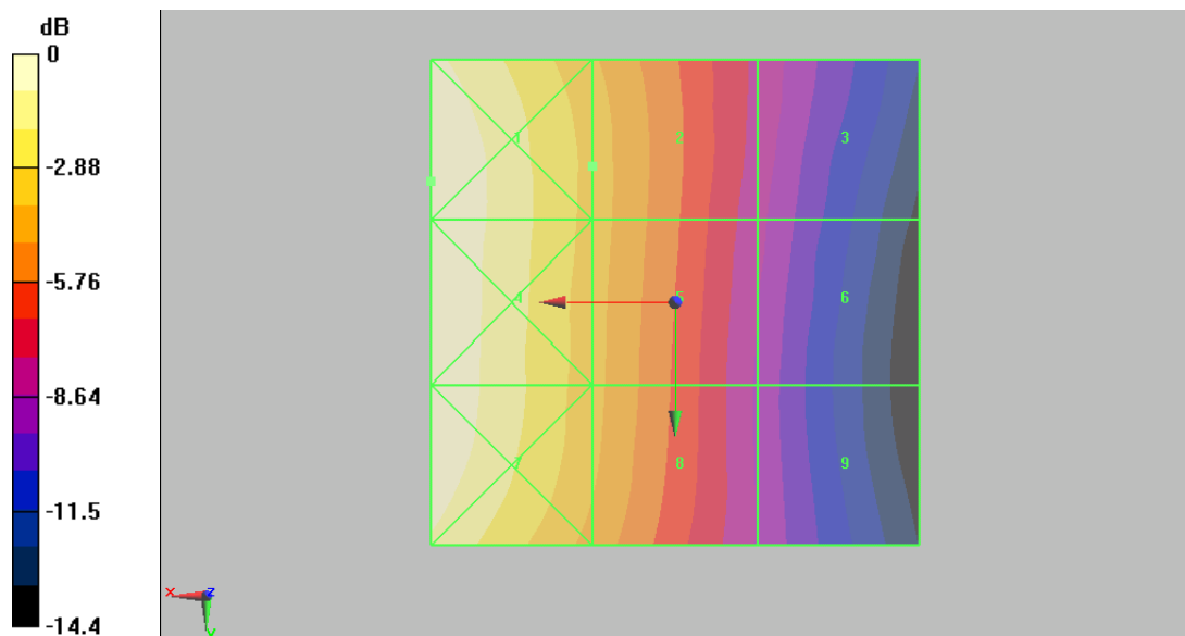
Figure 16 HAC RF H-Field GSM 850 Channel 190
