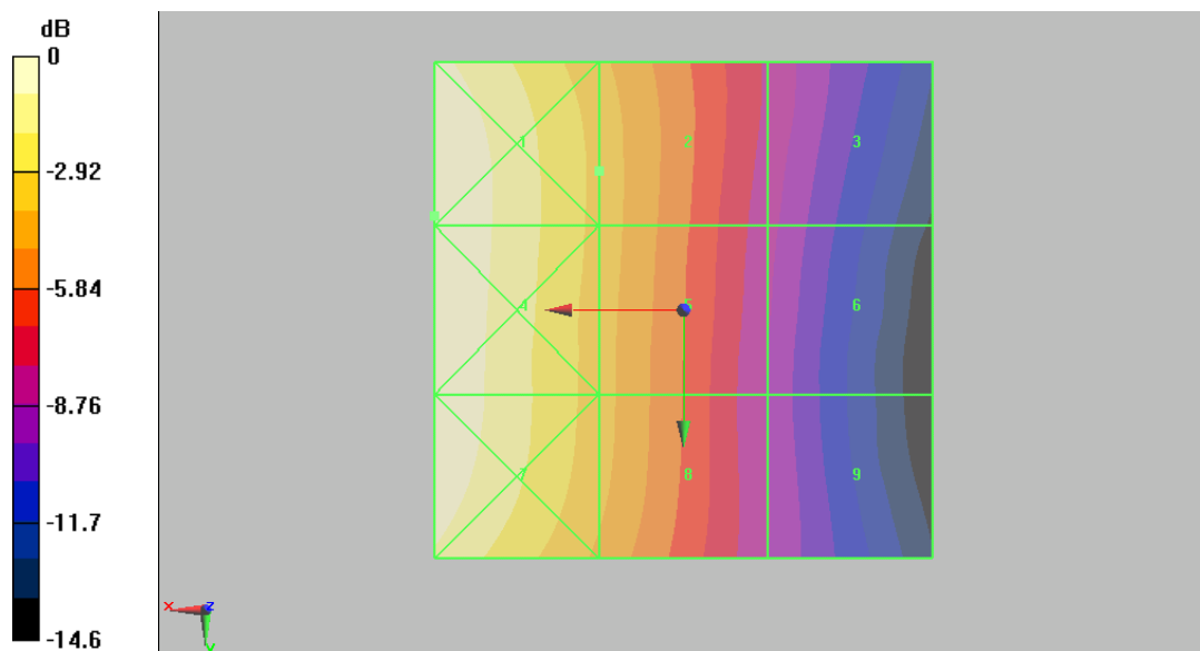
Figure 15 HAC RF H-Field GSM 850 Channel 251
