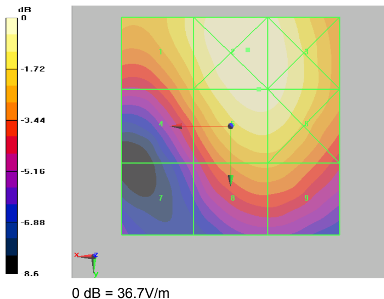
Figure 26 HAC RF E-Field WCDMA Band IV Channel 1312
