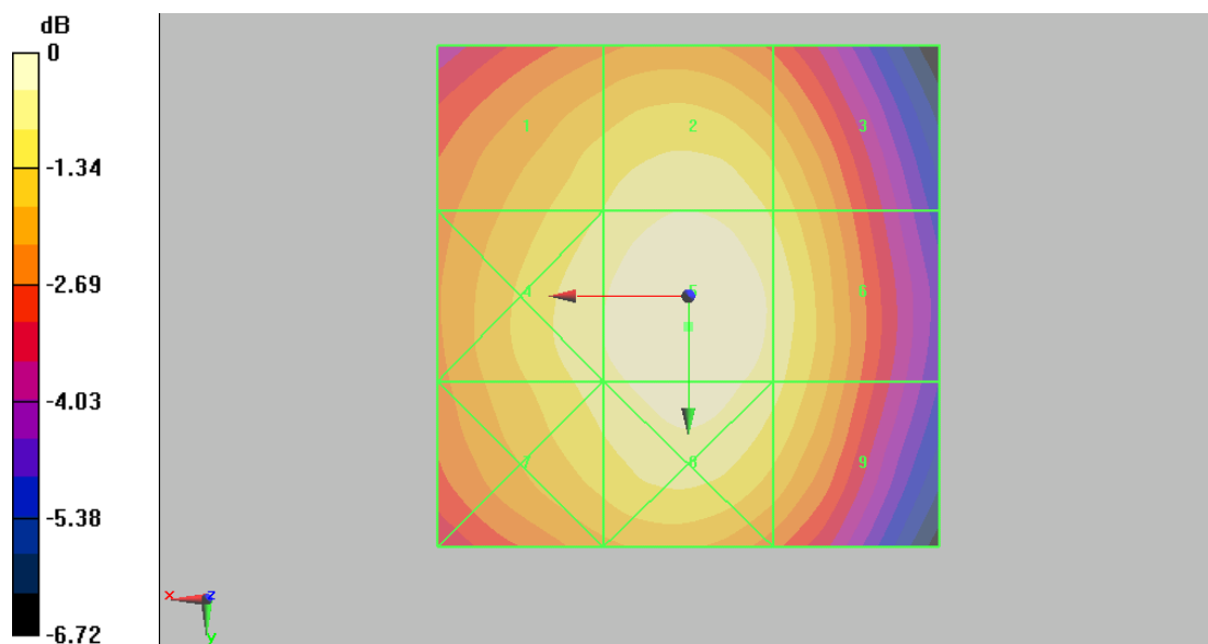
Figure 13 HAC RF E-Field GSM 850 Channel 190
