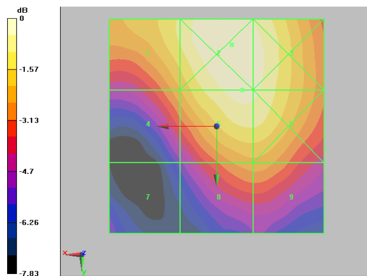
Figure 24 HAC RF E-Field WCDMA Band IV Channel 1513
