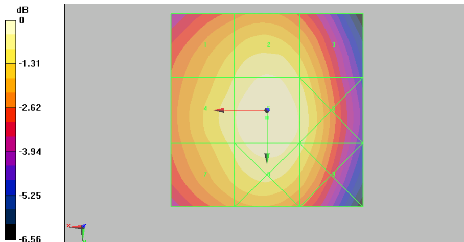
Figure 12 HAC RF E-Field GSM 850 Channel 251
