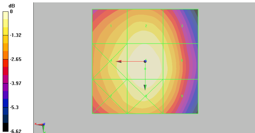
Figure 14 HAC RF E-Field GSM 850 Channel 128
