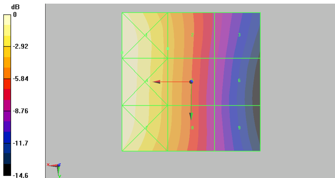
Figure 17 HAC RF H-Field GSM 850 Channel 128
