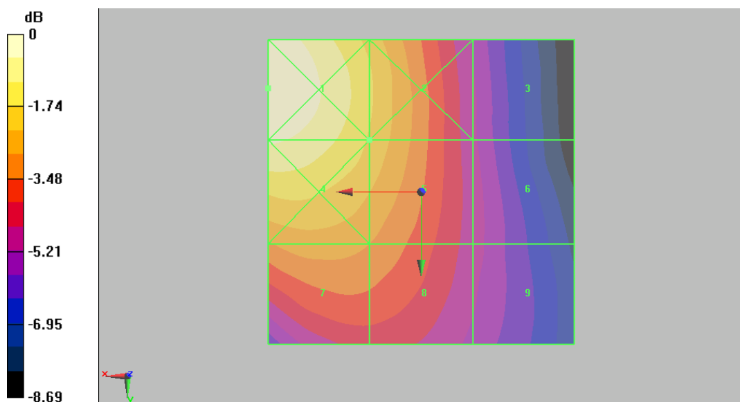
Figure 21 HAC RF H-Field GSM 1900 Channel 810
