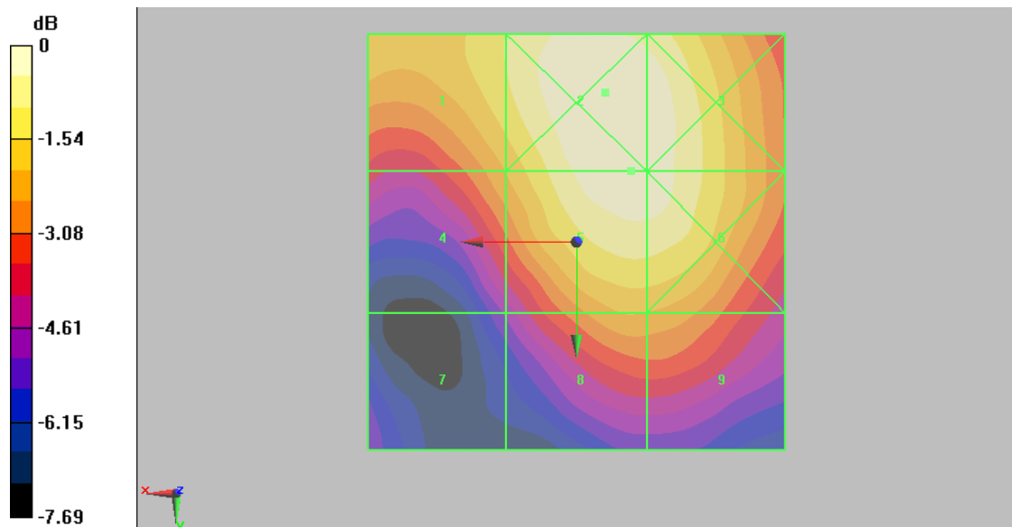
Figure 20 HAC RF E-Field GSM 1900 Channel 512
