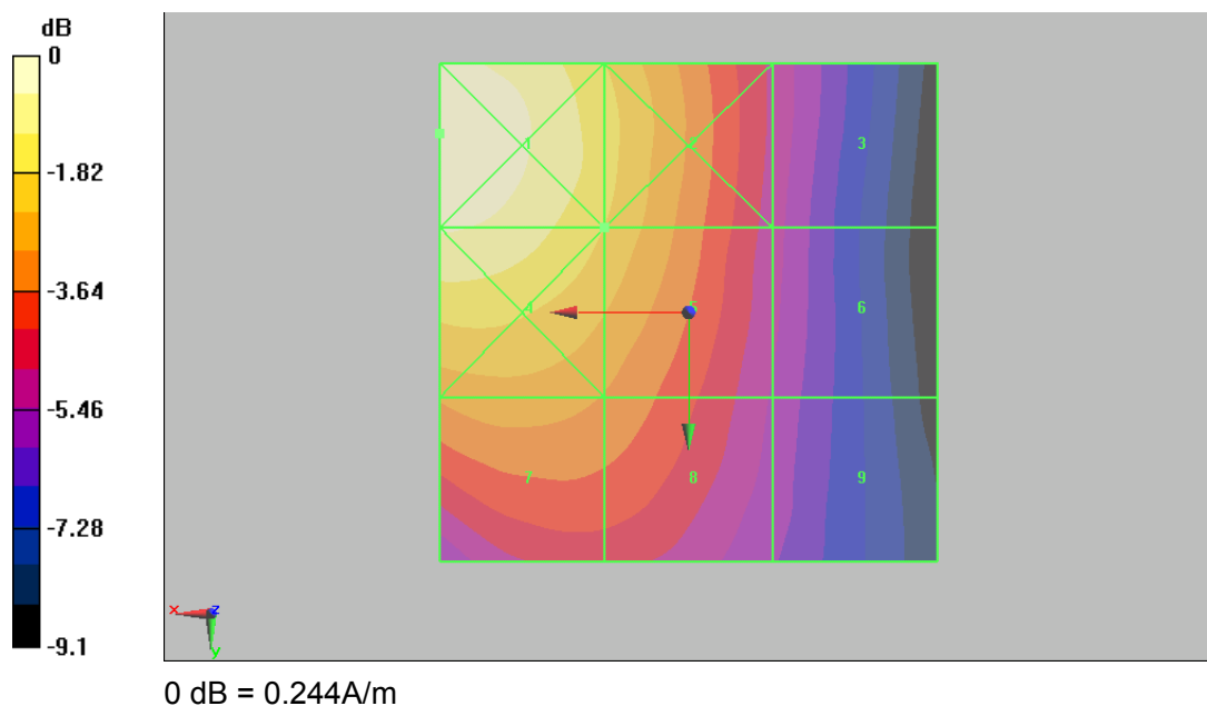
Figure 22 HAC RF H-Field GSM 1900 Channel 661
