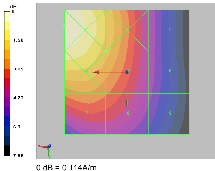
Figure 27 HAC RF H-Field WCDMA Band IV Channel 1513
