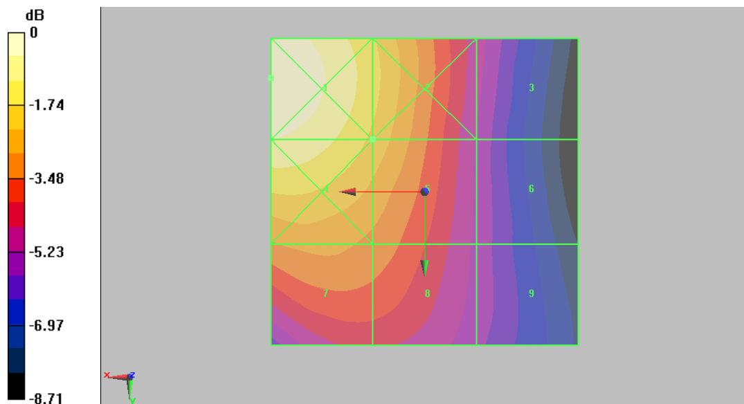
Figure 23 HAC RF H-Field GSM 1900 Channel 512
