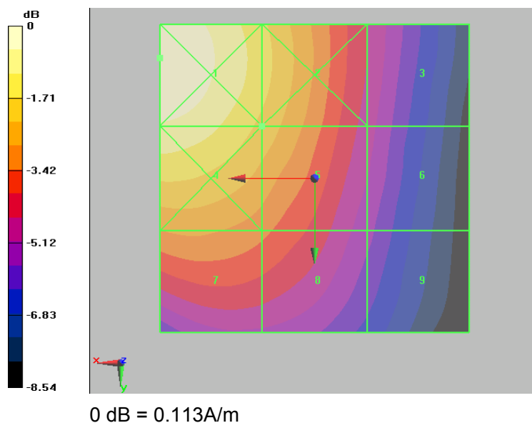
Figure 28 HAC RF H-Field WCDMA Band IV Channel 1413
