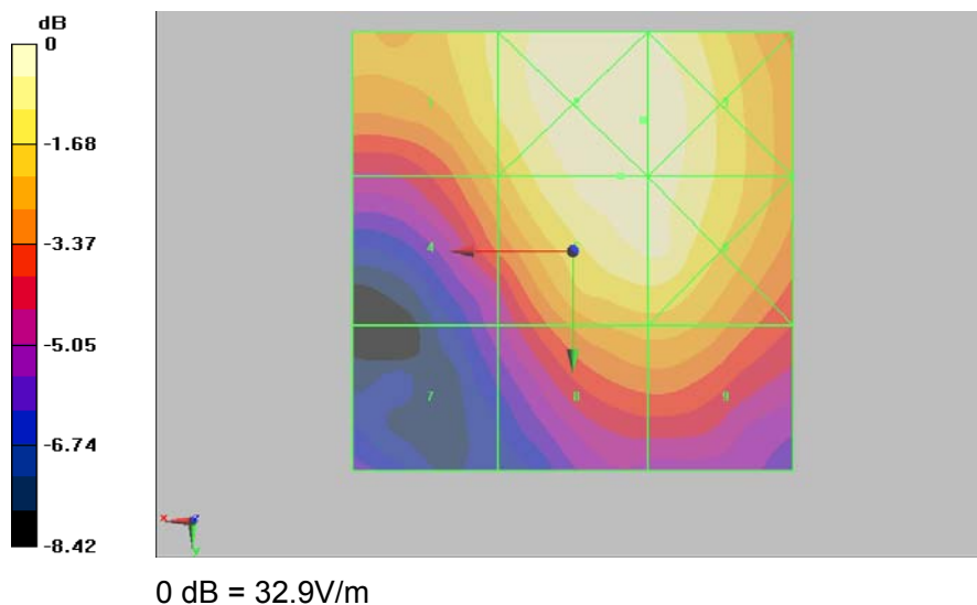
Figure 25 HAC RF E-Field WCDMA Band IV Channel 1413
