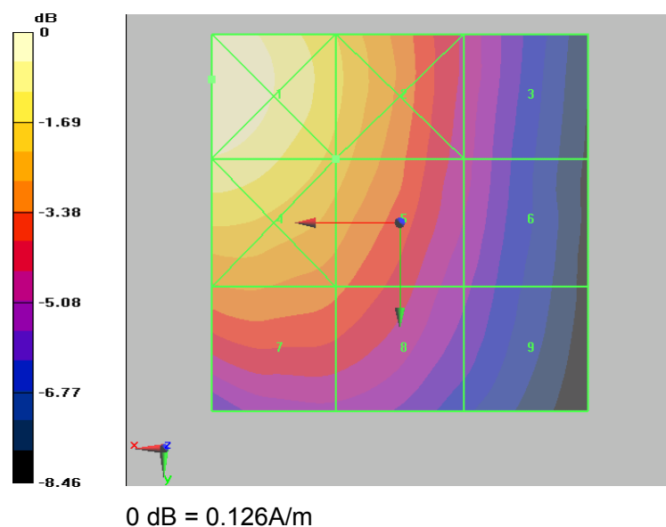
Figure 29 HAC RF H-Field WCDMA Band IV Channel 1312
