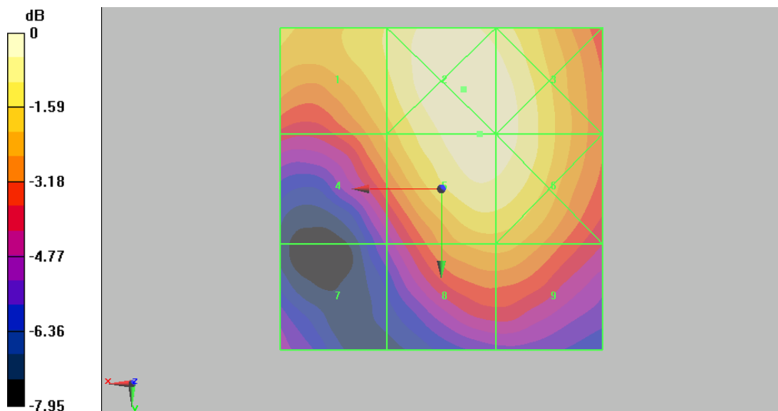
Figure 19 HAC RF E-Field GSM 1900 Channel 661
