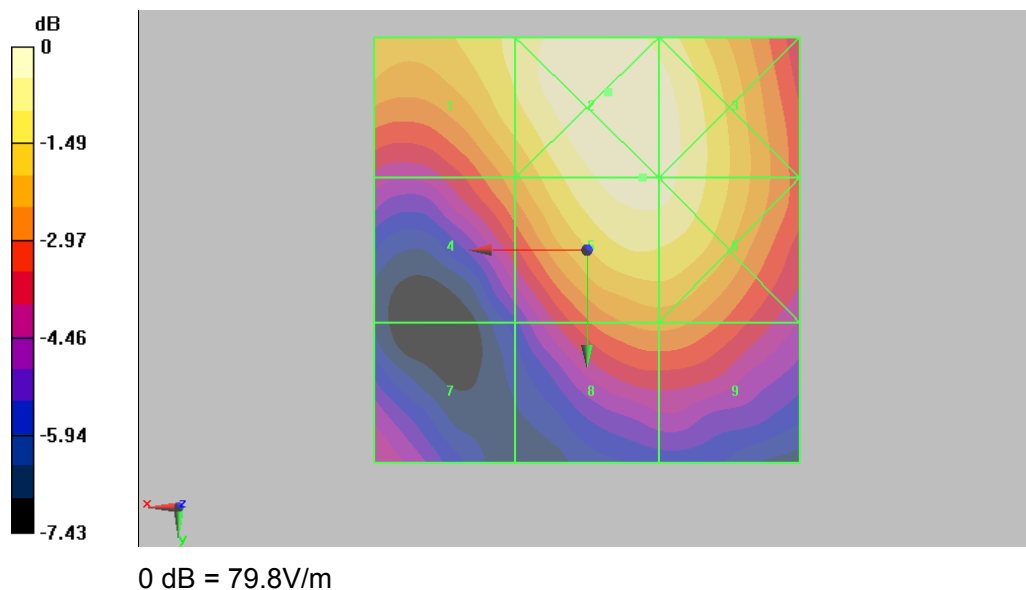
Figure 18 HAC RF E-Field GSM 1900 Channel 810
