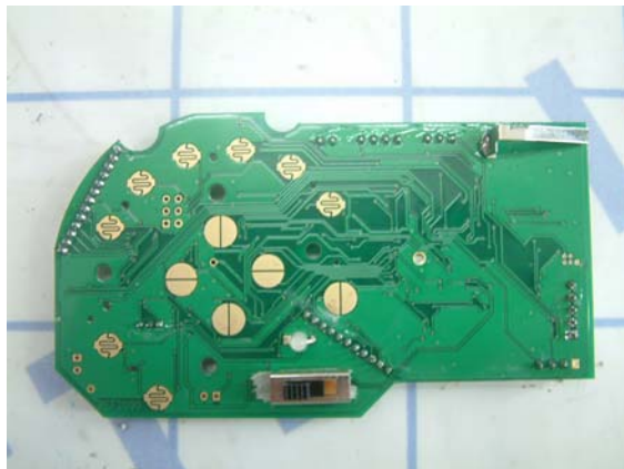
PCB layout-1
