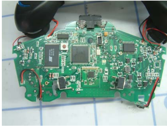
PCB layout-1
