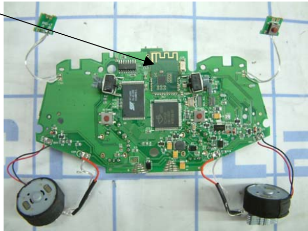
PCB Layout-1
