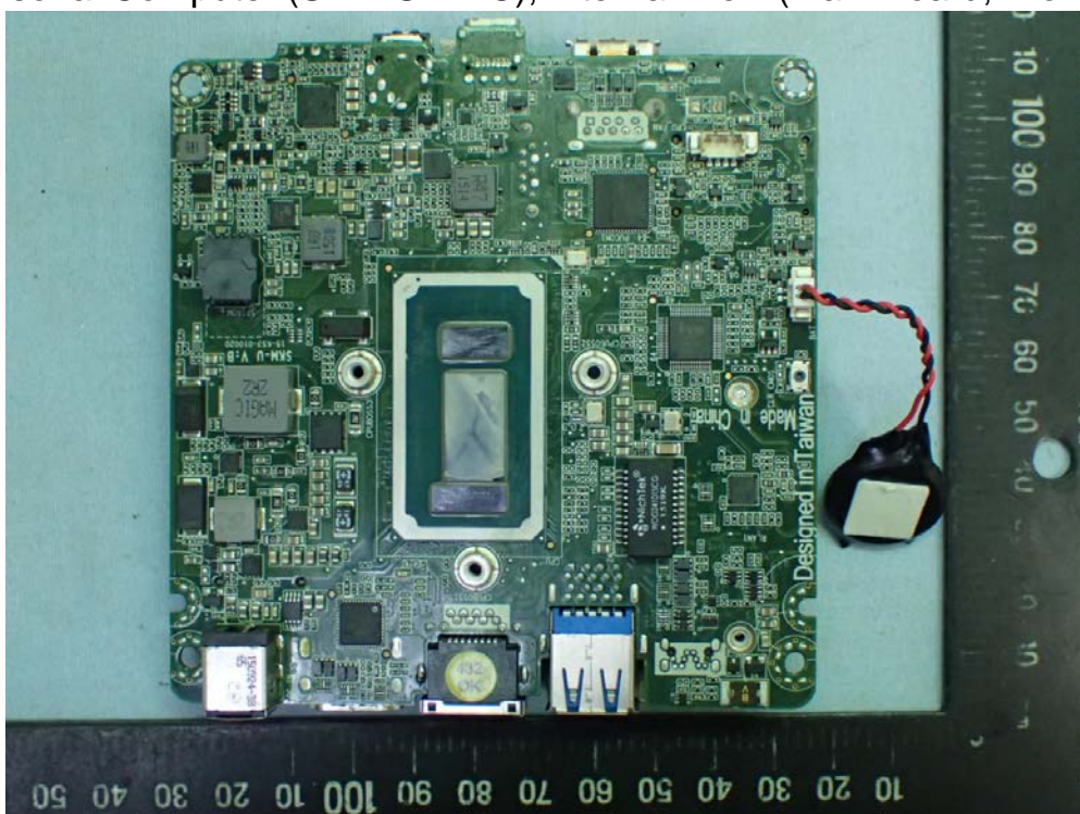
Figure 10 Personal Computer (SKM-U mPC), Internal View (Main Board, Front View)
