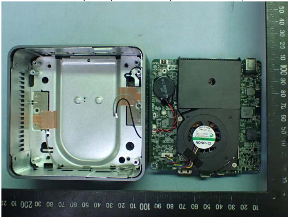
Figure 9 Personal Computer (SKM-U mPC), Internal View (Removed Cover)
