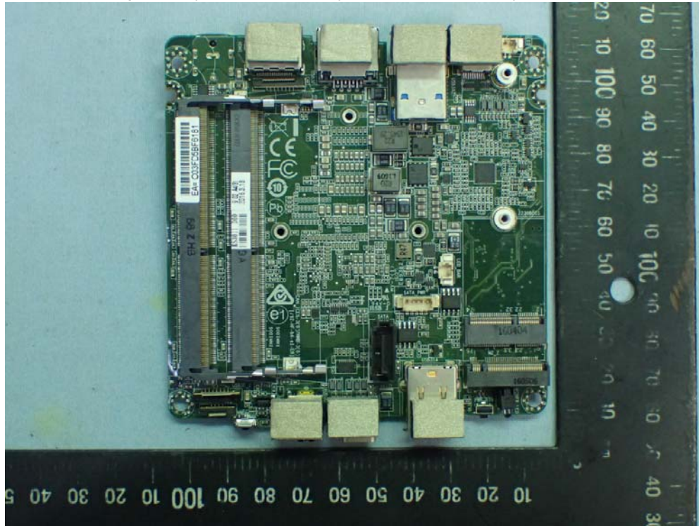
Figure 12 Personal Computer (SKM-U mPC), Internal View
