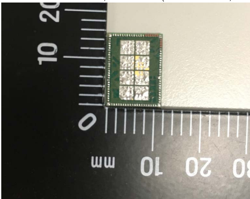
7" Multi Function Pad, Internal View (Wireless Module, Back View)
