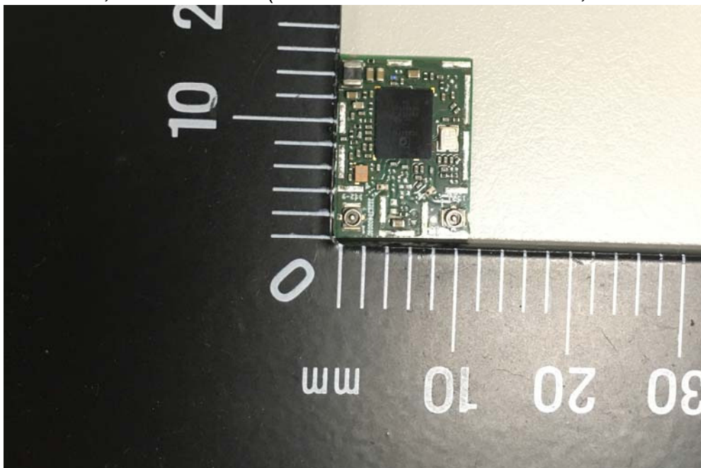
7" Multi Function Pad, Internal View (Wireless Module/Front View, Removed Cover)
