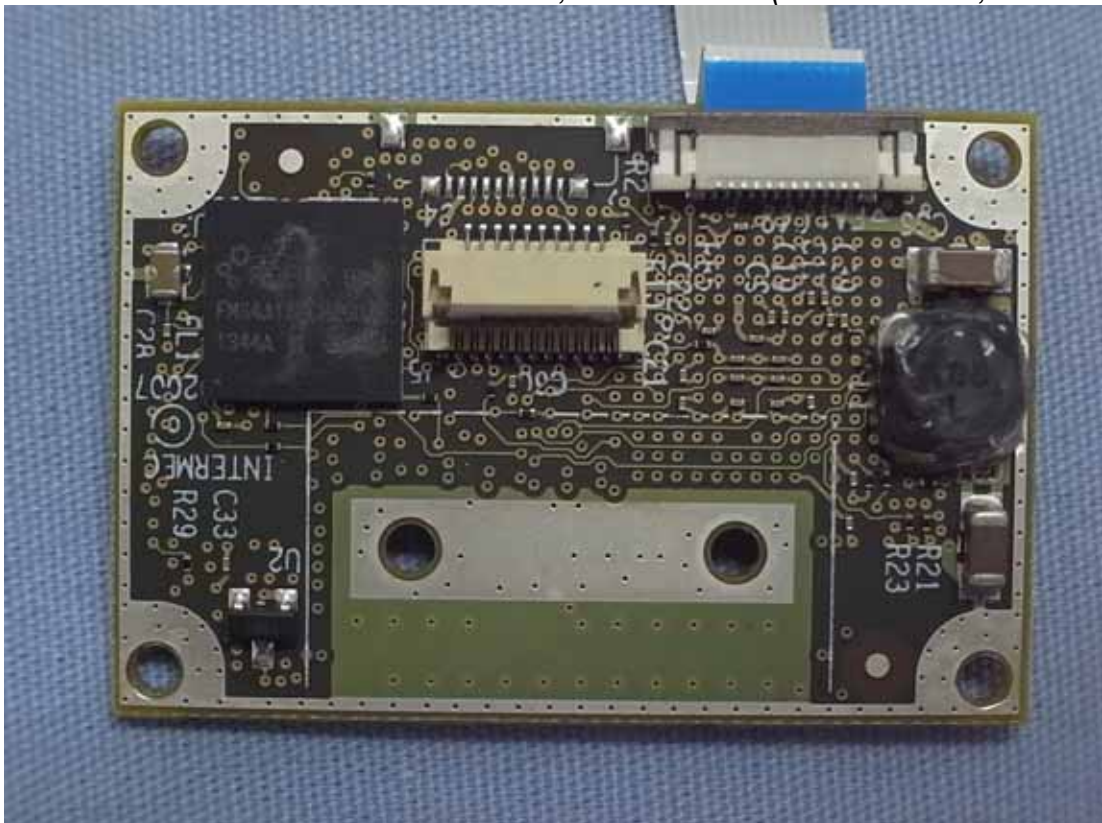
Figure 38 7" Pocketable Pad, Internal View (Control Board, Back View)
