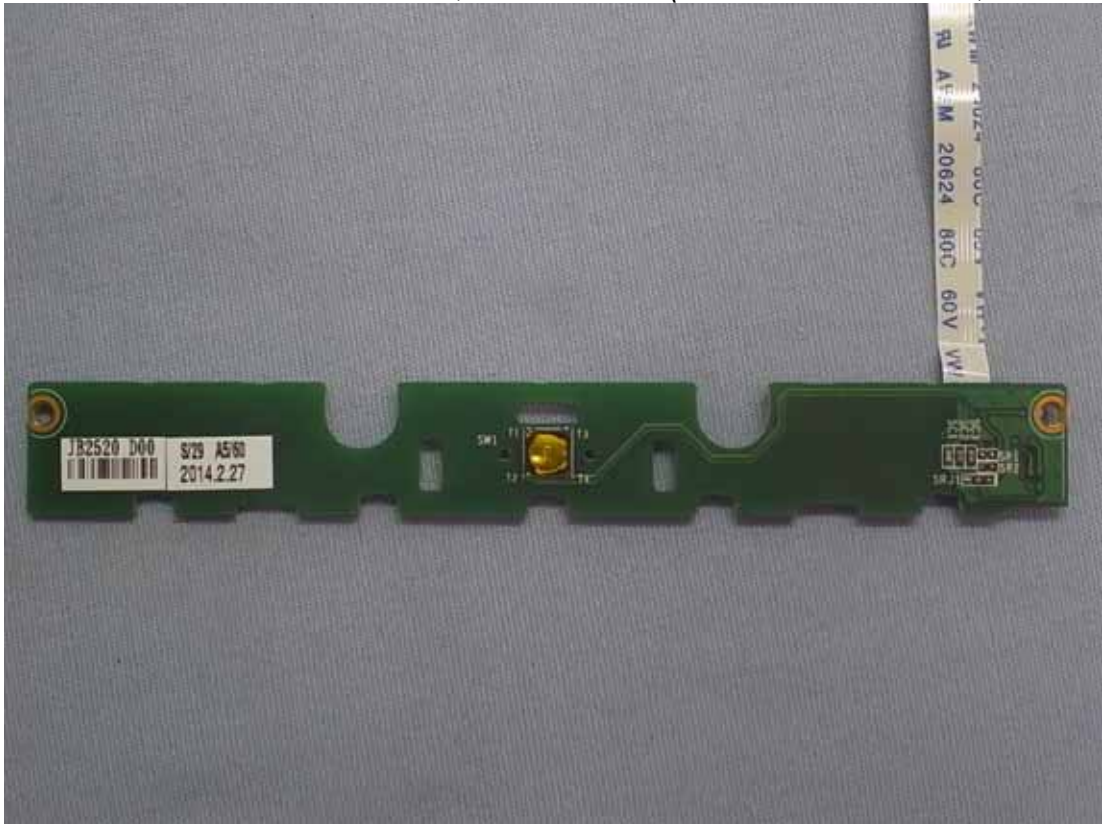
Figure 49 7" Pocketable Pad, Internal View (Button Control Board, Back View)
