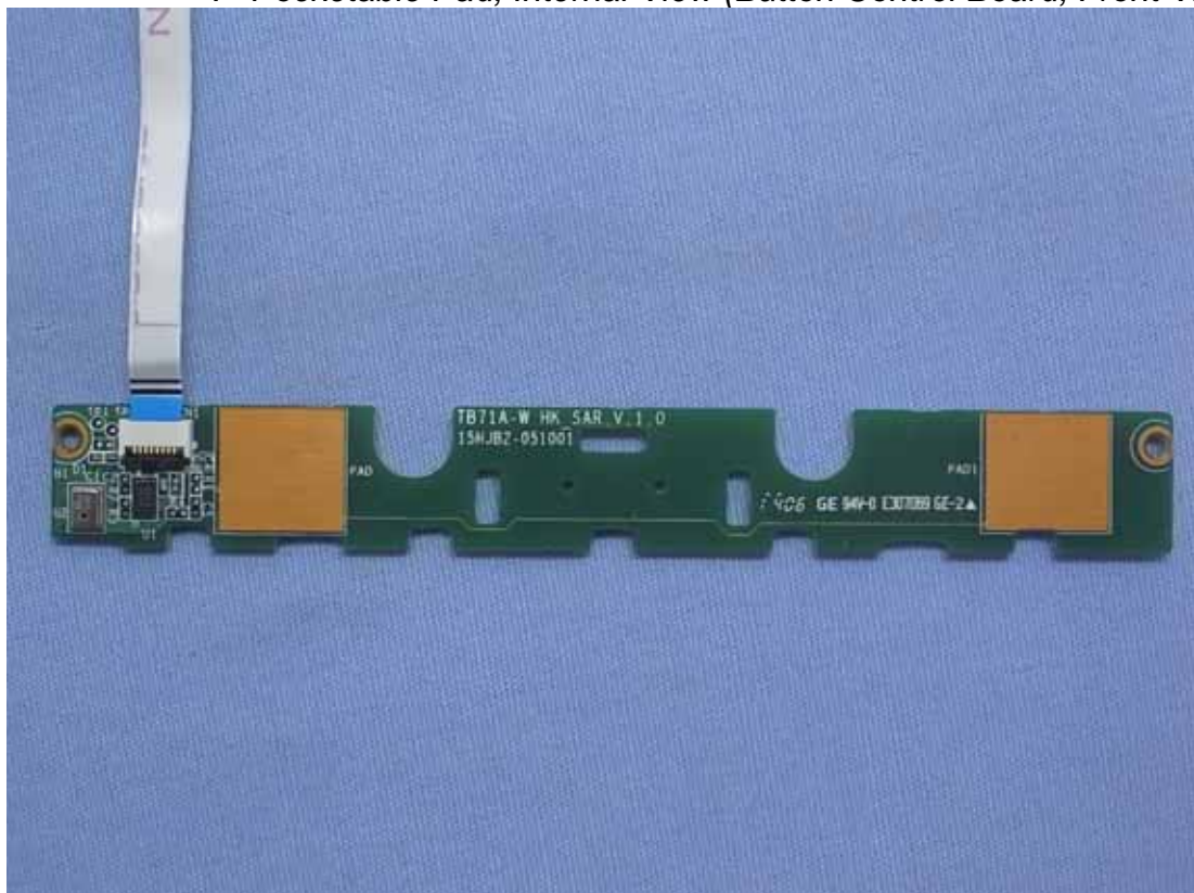
7" Pocketable Pad, Internal View (Button Control Board, Front View)
