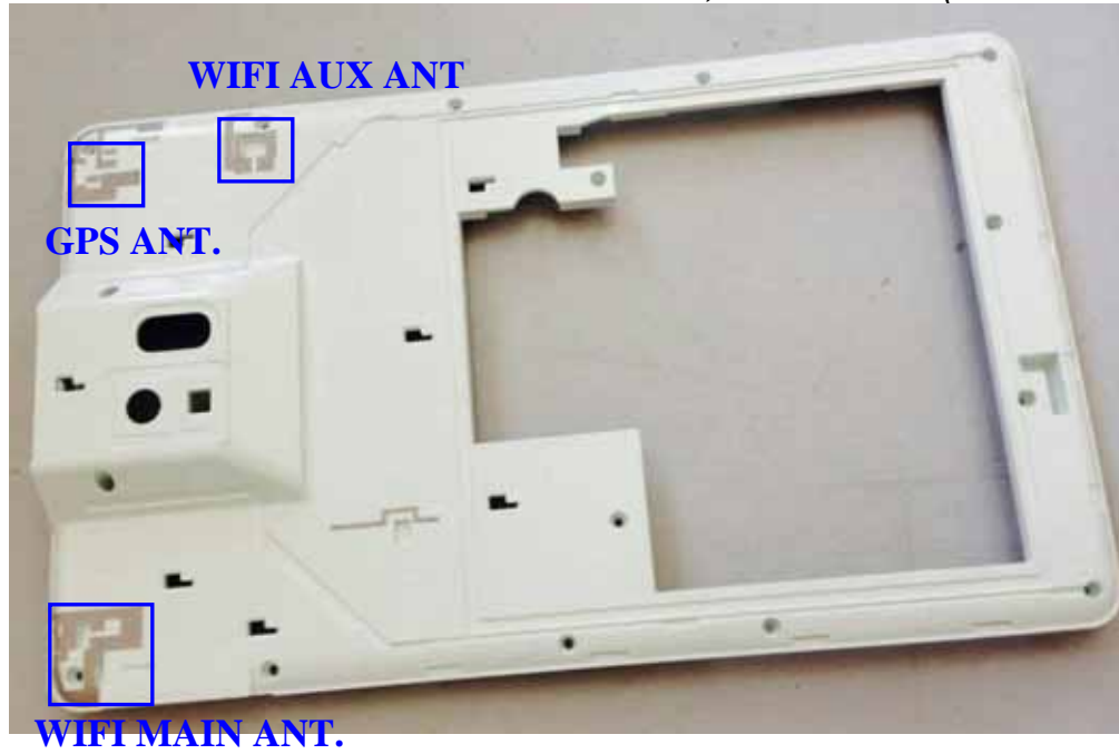
Figure 54 7" Pocketable Pad, Internal View (Antenna View)
