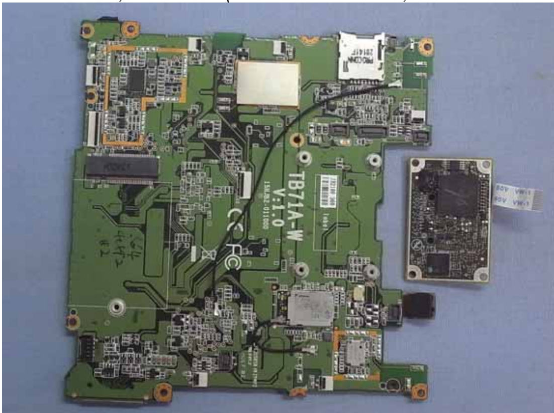
Figure 36 7" Pocketable Pad, Internal View (Removed Control Board, Main Board/Front View)
