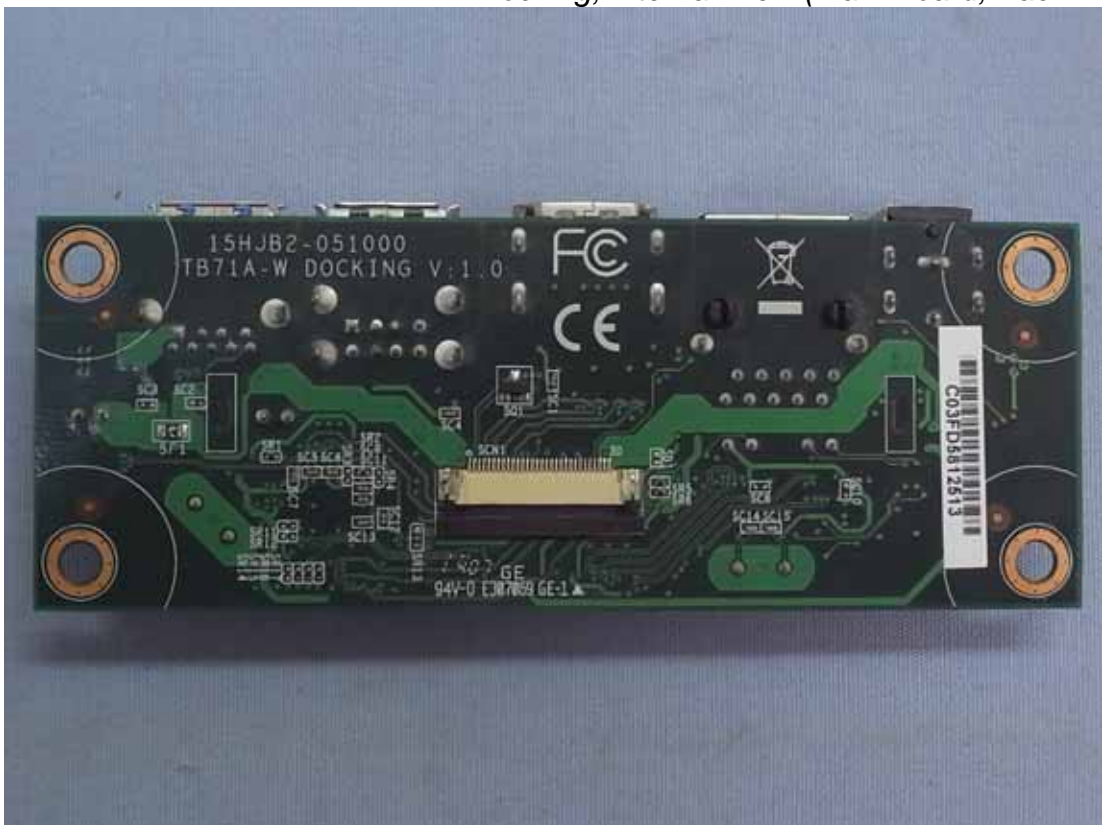
Figure 58 Docking, Internal View (Main Board, Back View)
