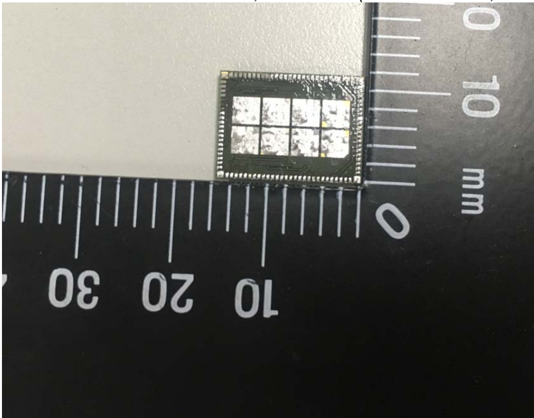
7" Multi Function Pad, Internal View (Wi-Fi +BT Module, Back View)
