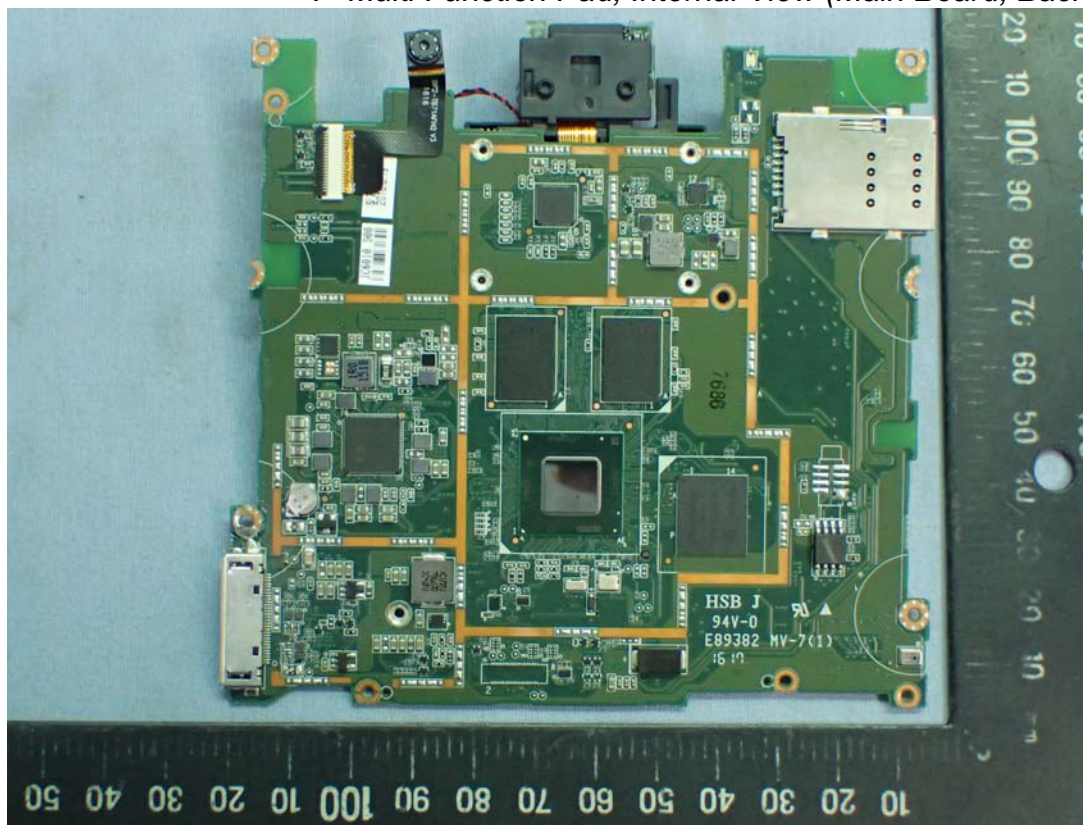
Figure 30 7" Multi Function Pad, Internal View (Main Board, Back View)
