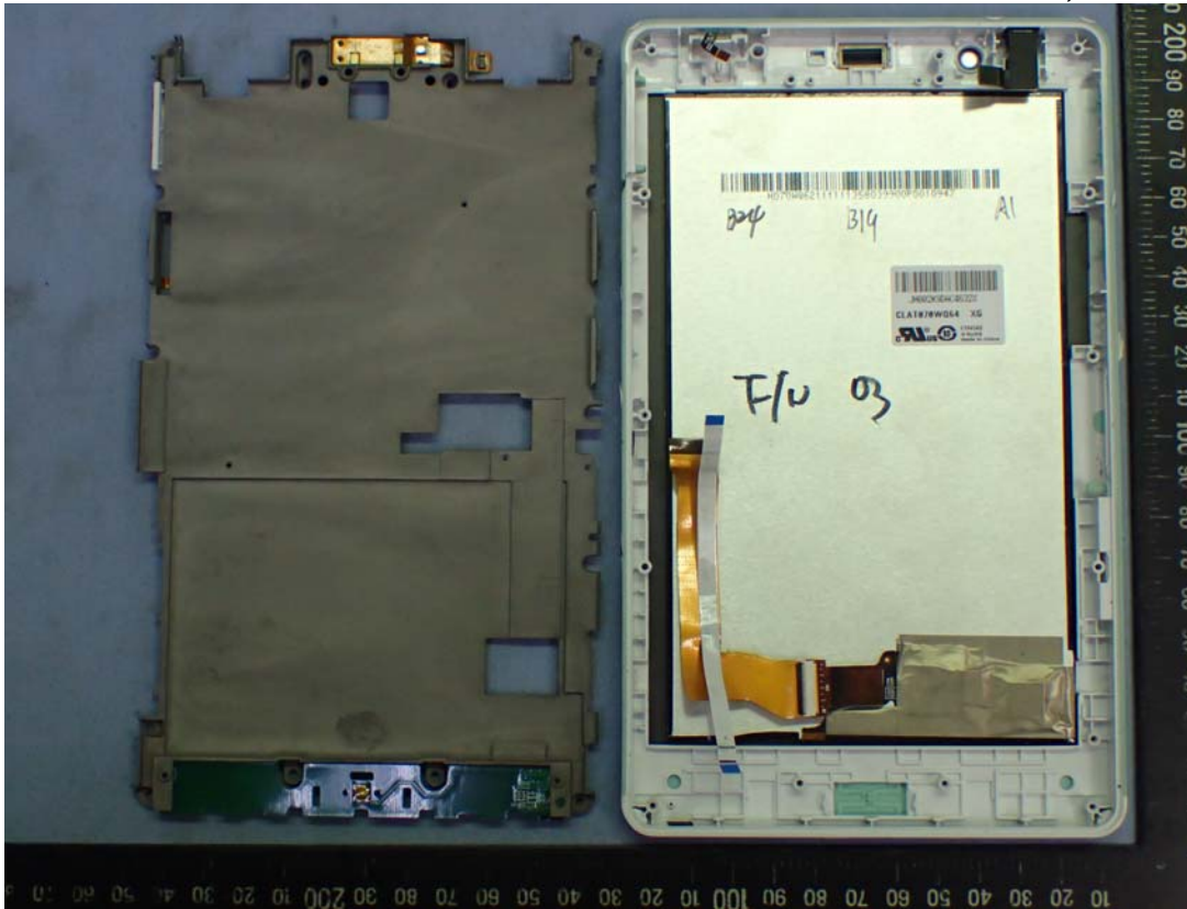
Figure 37 7" Multi Function Pad, Internal View
