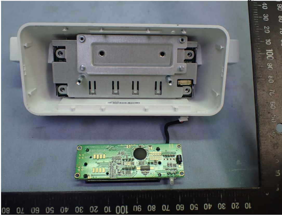
Figure 45 7" Pad Docking, Internal View
