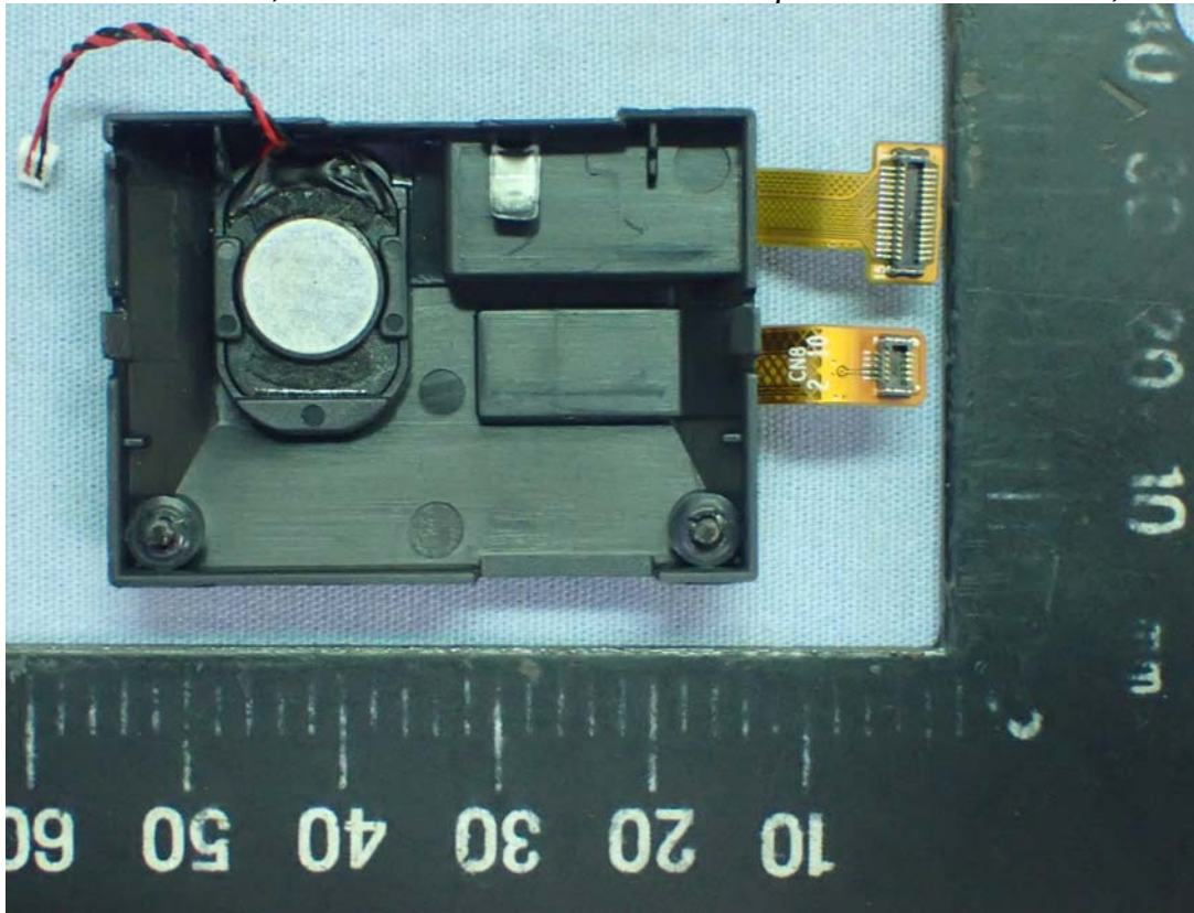
7" Multi Function Pad, Internal View WEB CAM and Speaker Control Board, Back View
