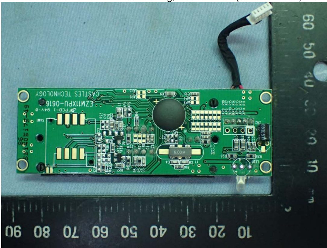
Figure 46 7" Pad Docking, Internal View (Control Board, Front View)
