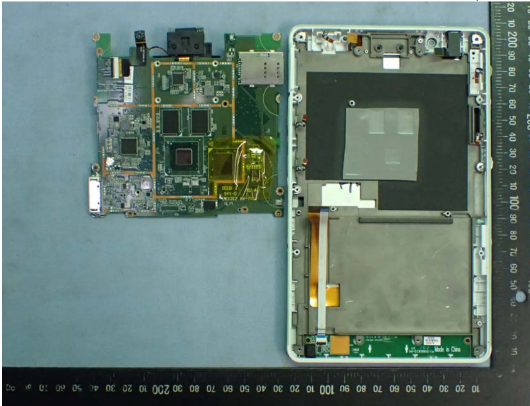
Figure 21 7" Multi Function Pad, Internal View
