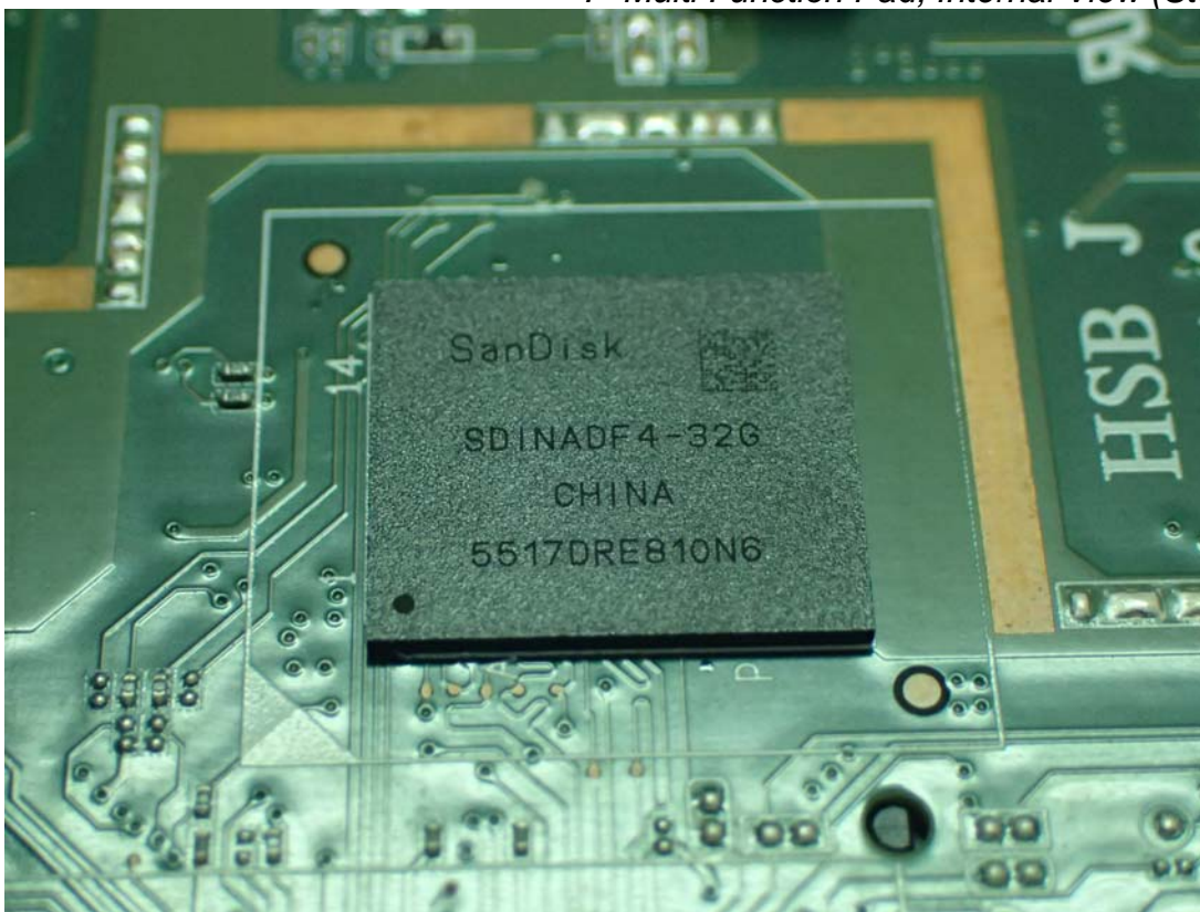
Figure 32 7" Multi Function Pad, Internal View (Storage)
