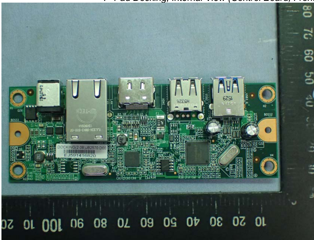
Figure 50 7" Pad Docking, Internal View (Control Board, Front View)
