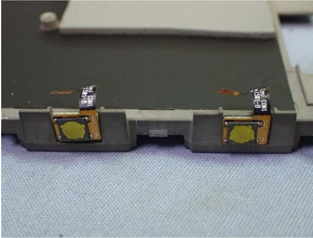
Figure 41 7" Multi Function Pad, Internal View
