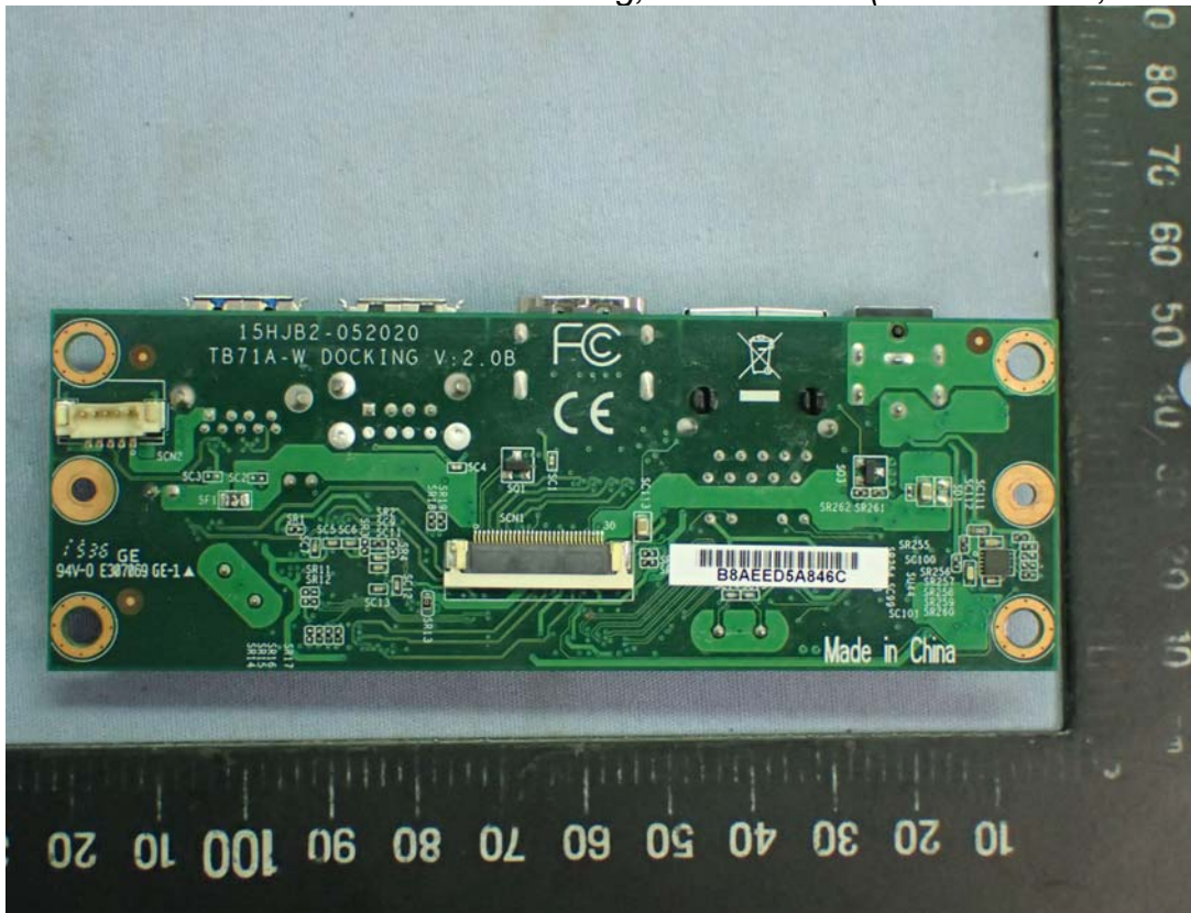
Figure 49 7" Pad Docking, Internal View (Control Board, Back View)
