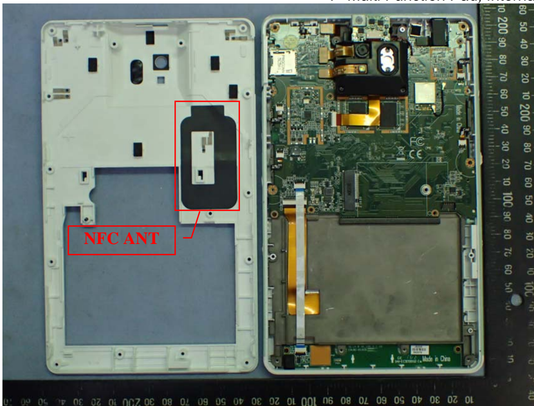
Figure 20 7" Multi Function Pad, Internal View
