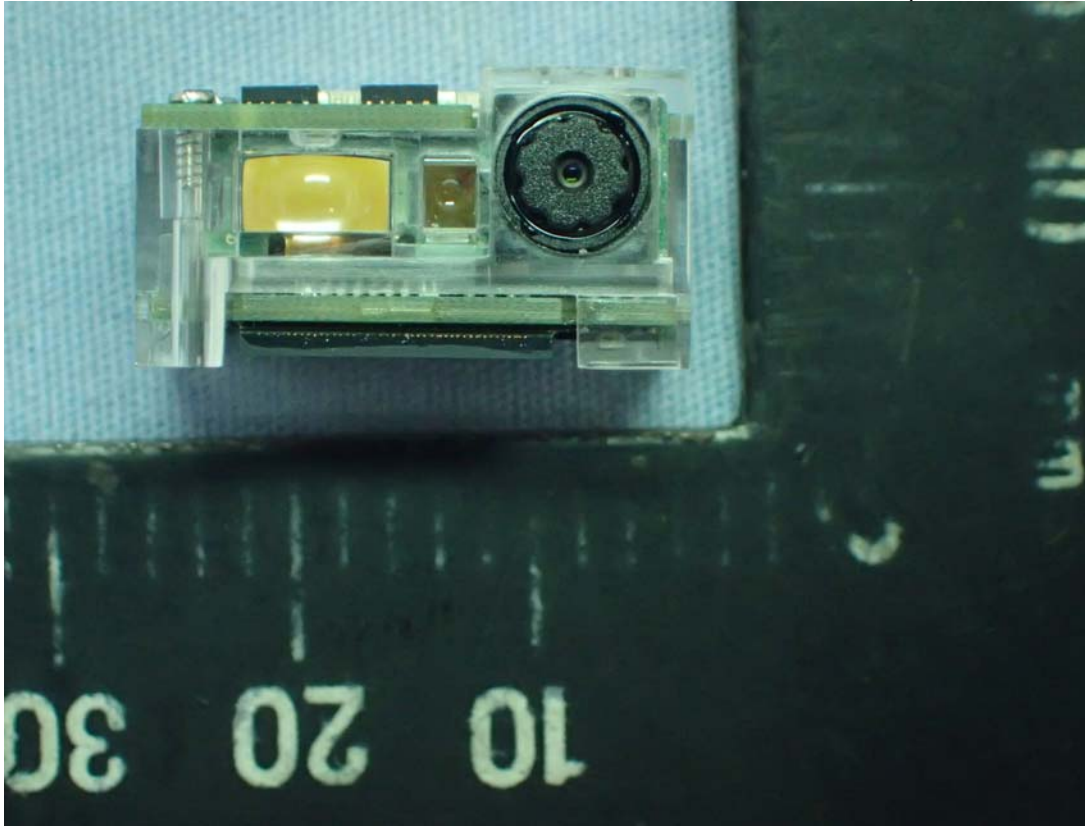
Figure 27 7" Multi Function Pad, Internal View (Barcode Scanner)
