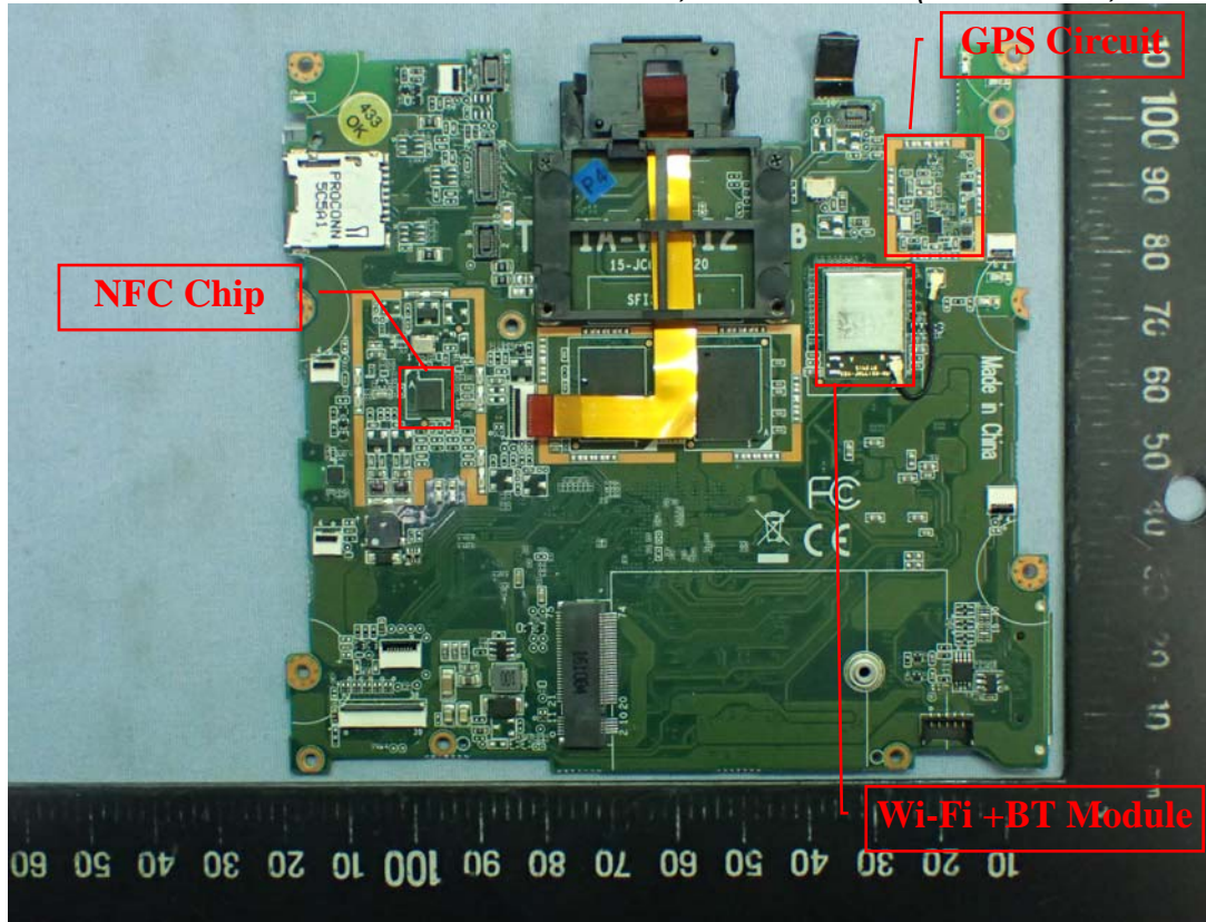
Figure 29 7" Multi Function Pad, Internal View (Main Board, Front View)
