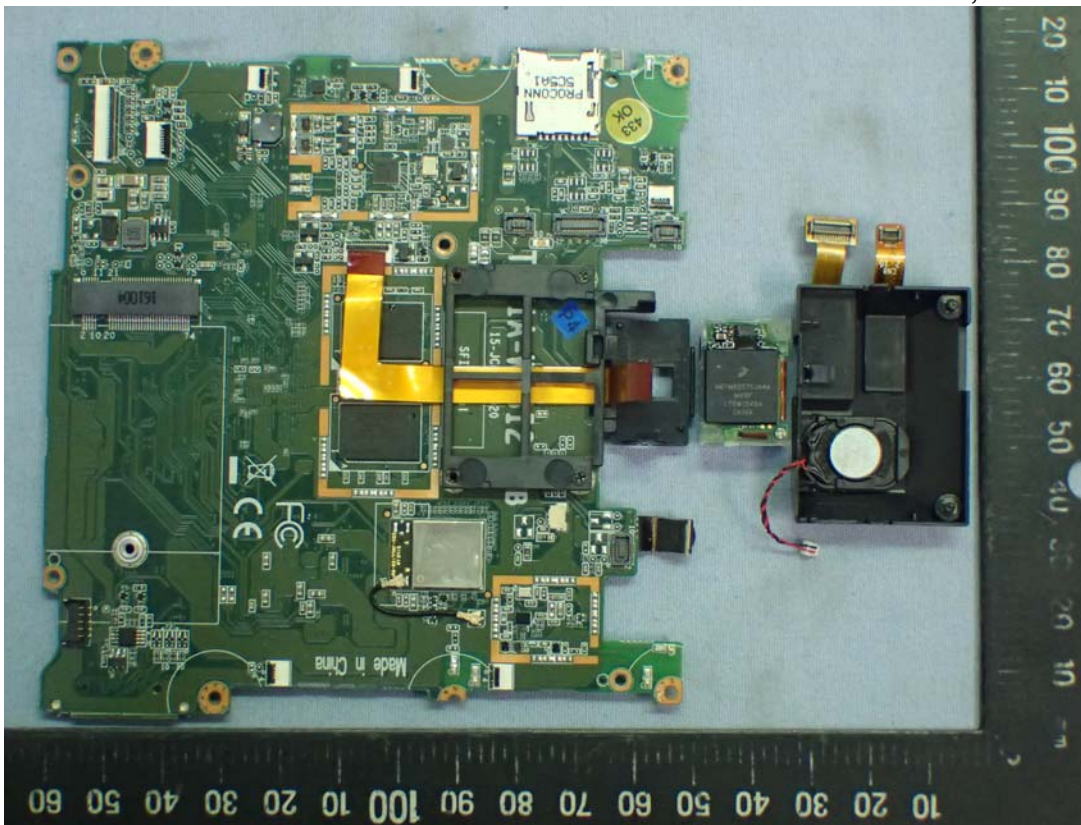
Figure 22 7" Multi Function Pad, Internal View
