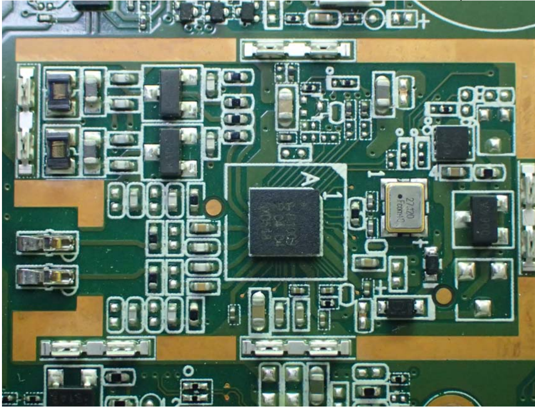
Figure 51 7" Multi Function Pad, Internal View (NFC Schematic)
