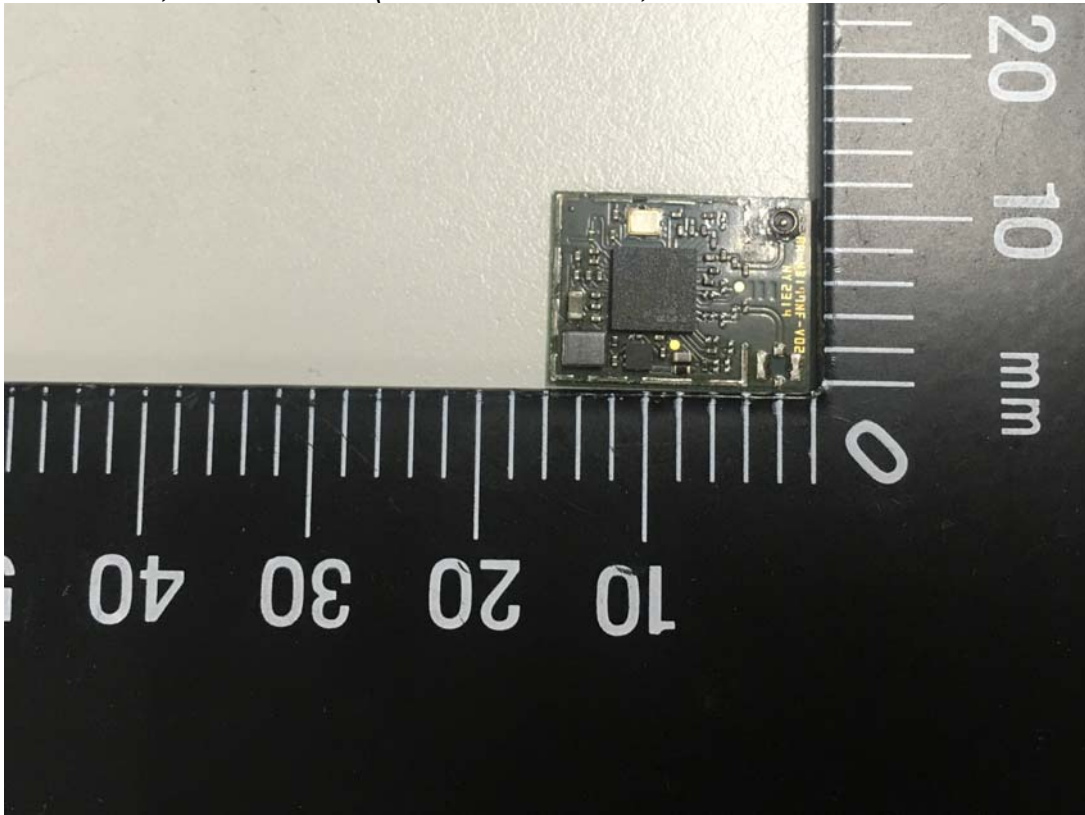
7" Multi Function Pad, Internal View (Wi-Fi +BT Module, Front View/Removed Shielded Case)
