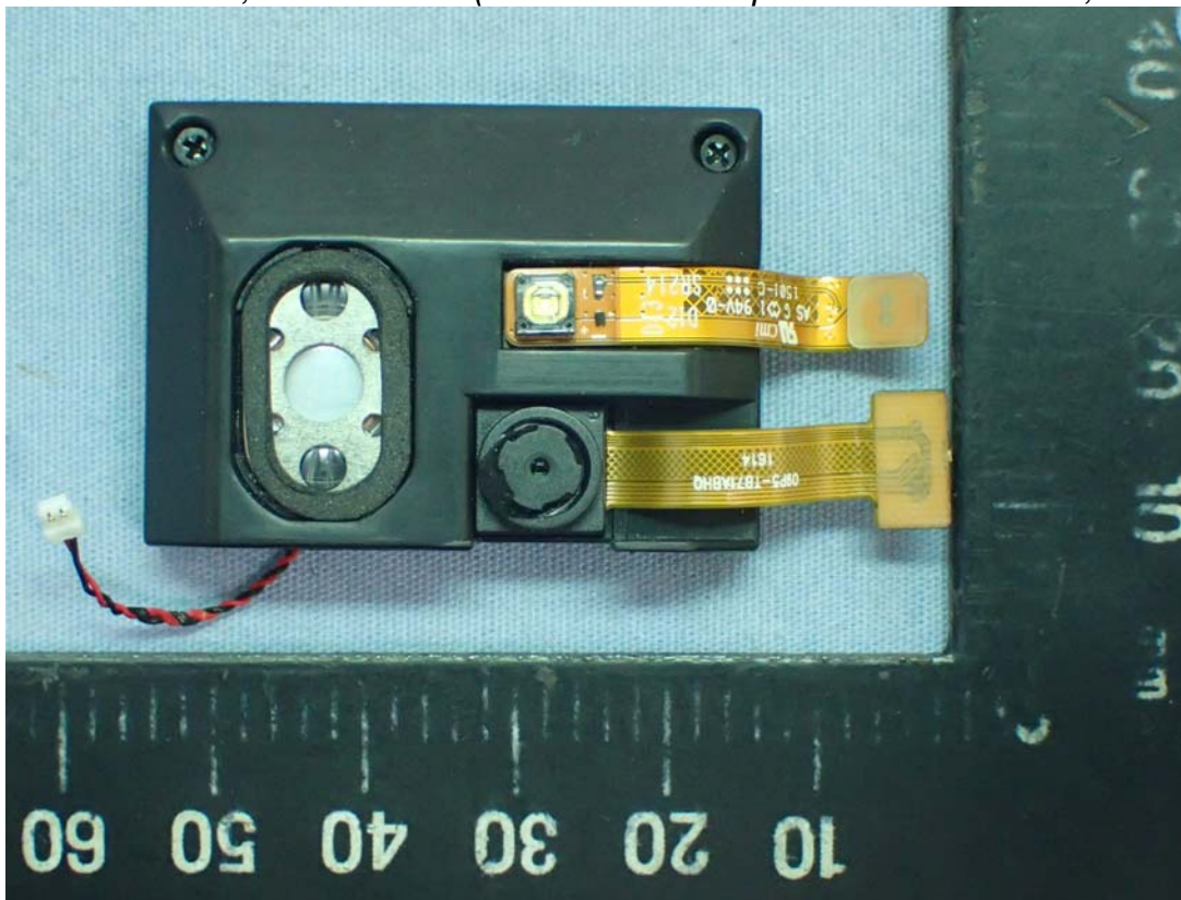
7" Multi Function Pad, Internal View (WEB CAM and Speaker Control Board, Front View)
