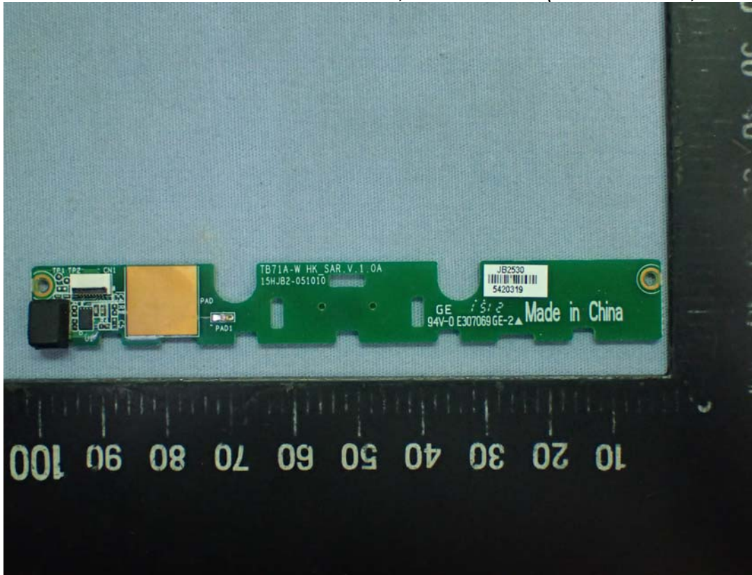
Figure 39 7" Multi Function Pad, Internal View (Control Board, Front View)
