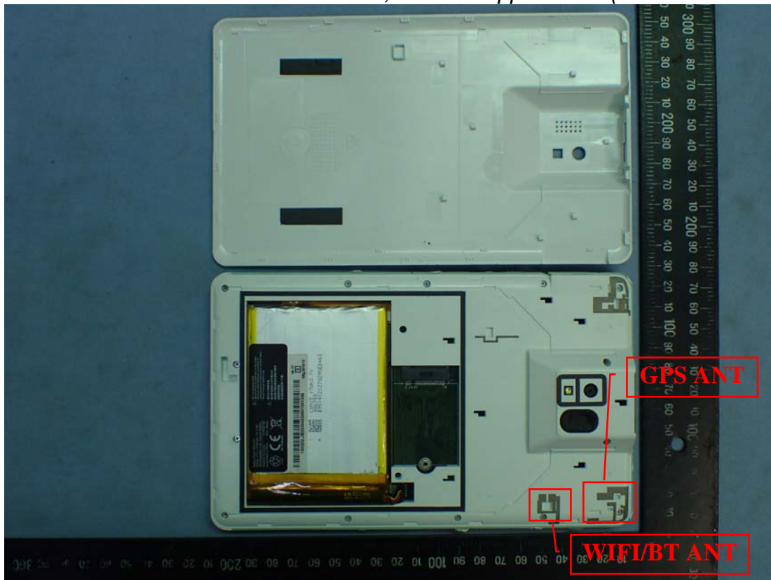
Figure 17 7" Multi Function Pad, General Appearance (Remove Back Cover)
