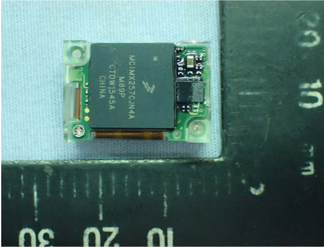
Figure 25 7" Multi Function Pad, Internal View (Barcode Scanner)
