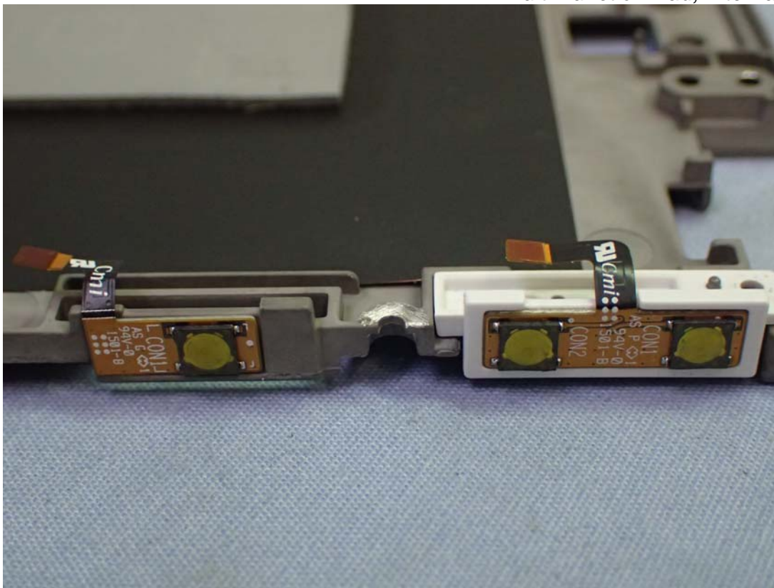
Figure 42 7" Multi Function Pad, Internal View
