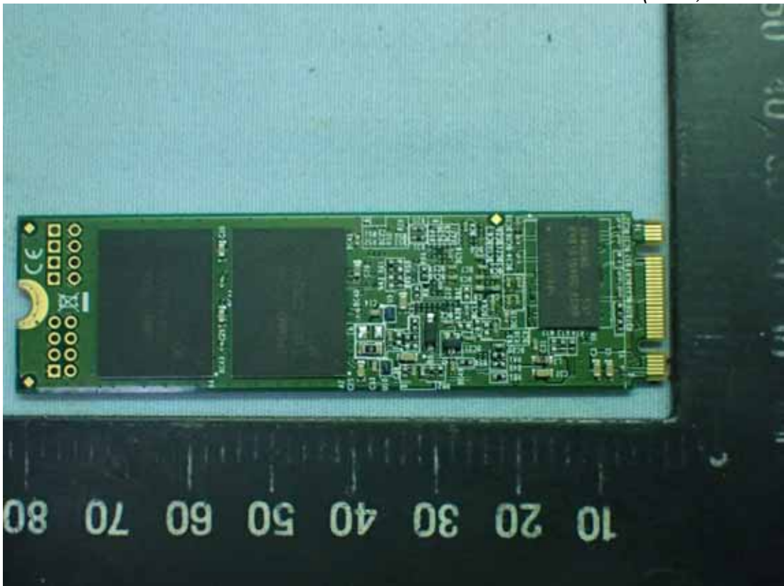
Figure 27 Internal View (SSD, Back View)
