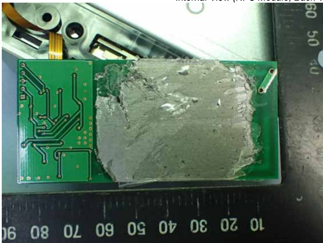
Figure 33 Internal View (NFC Module, Back View)
