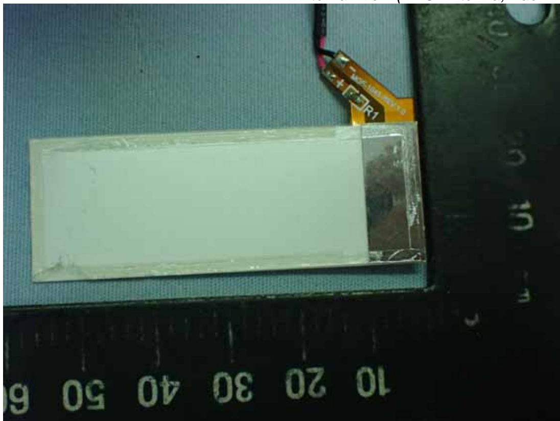
Figure 35 Internal View (NFC Antenna, Back View)
