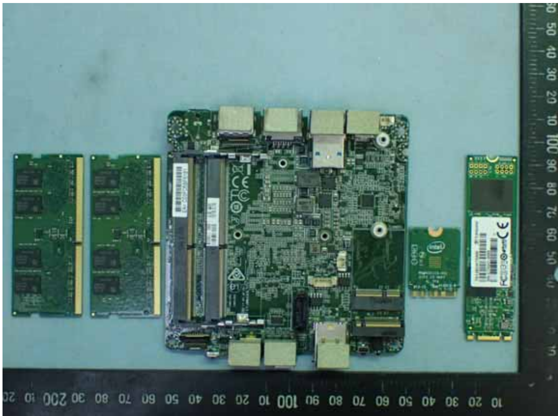
Figure 22 Internal View
