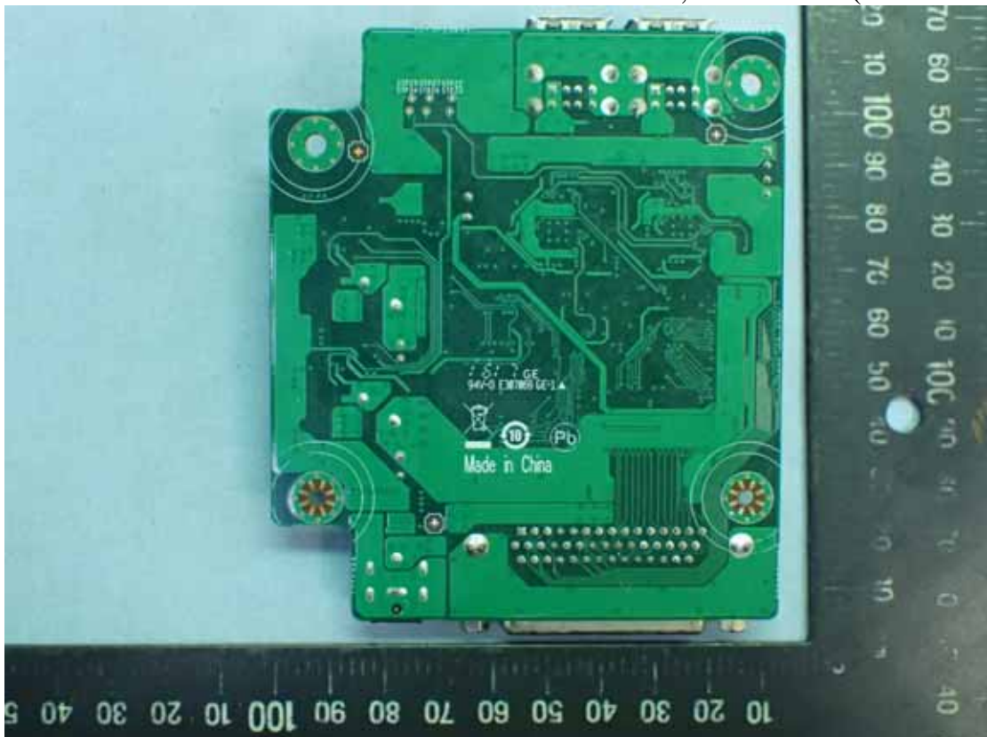
Figure 54 COM Box, Main Board (Back View)
