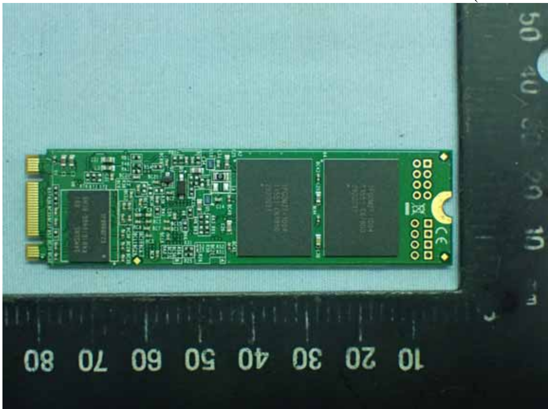
Figure 30 SSD (Back View)
