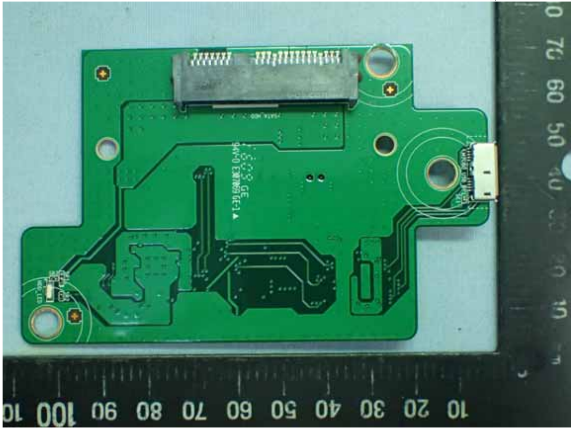
Figure 45 HDD Box, Main Board (Front View)
