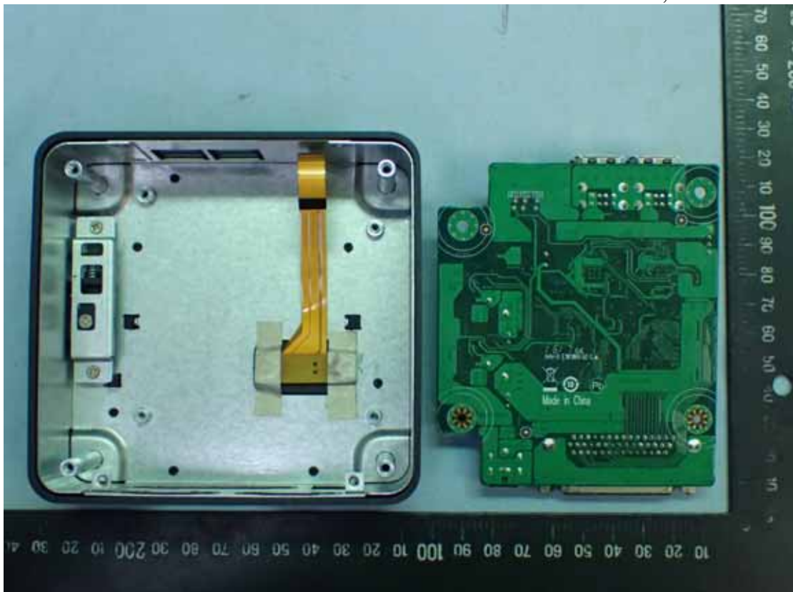
Figure 52 COM Box, Internal View
