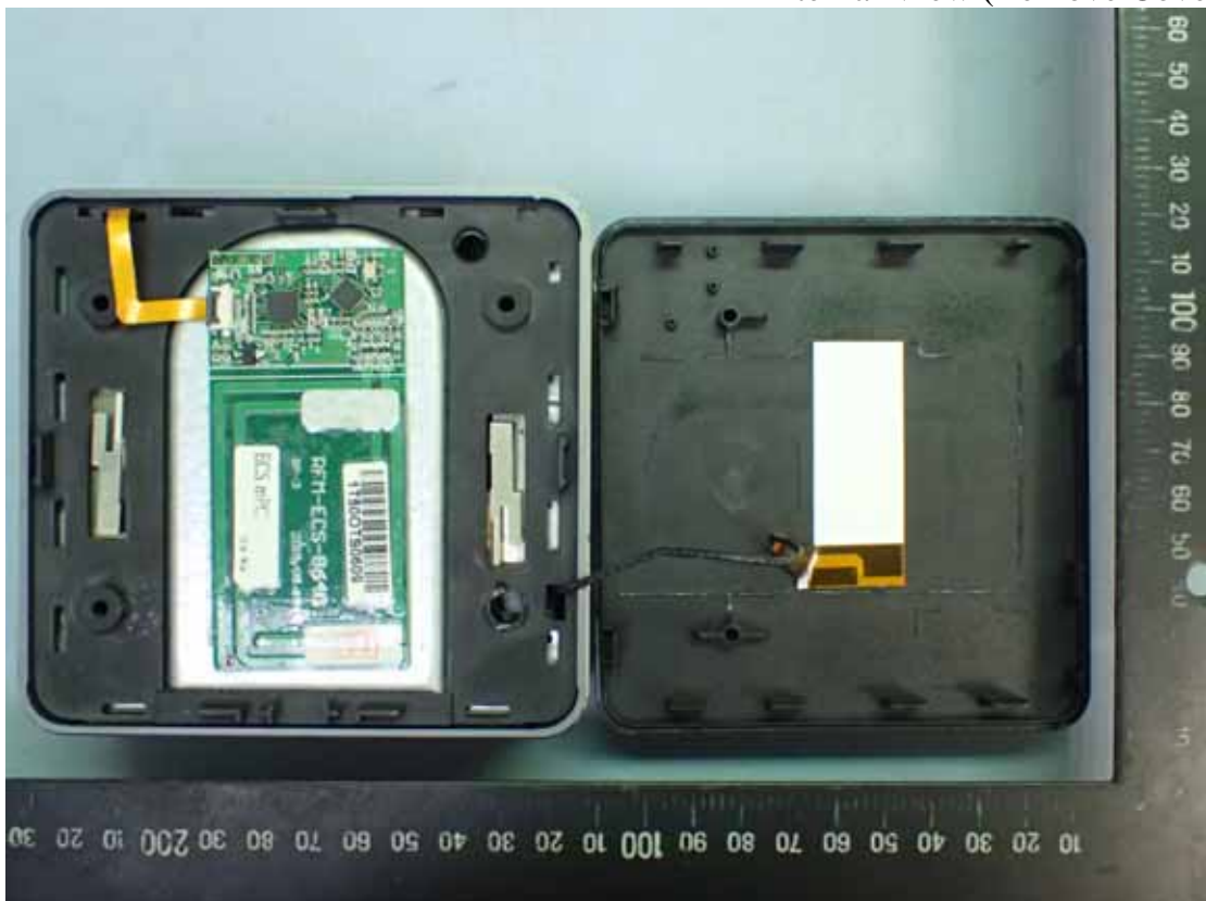
Figure 16 Internal View (Remove Cover)
