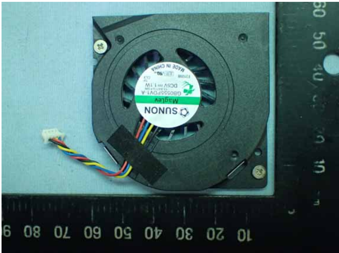
Figure 26 Fan View
