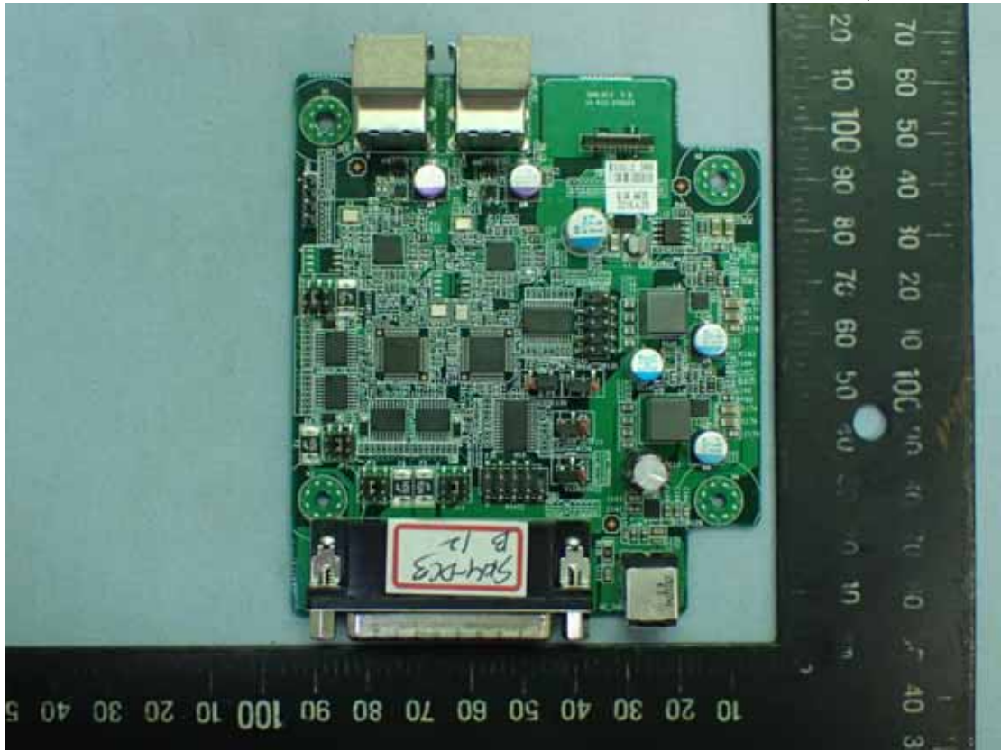
Figure 53 COM Box, Main Board (Front View)
