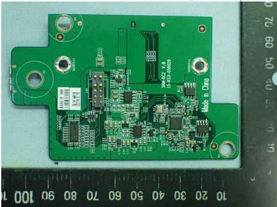
Figure 46 HDD Box, Main Board (Back View)
