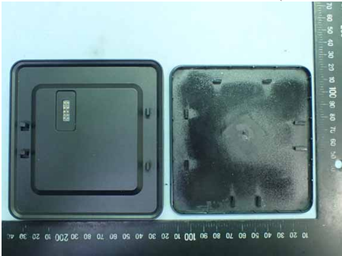
Figure 41 HDD Box (Remove Cover)
