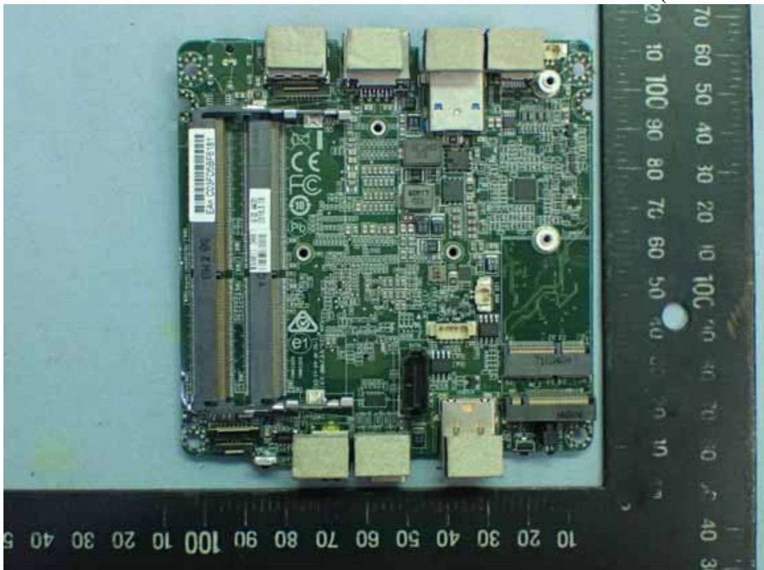
Figure 24 Main Board (Back View)
