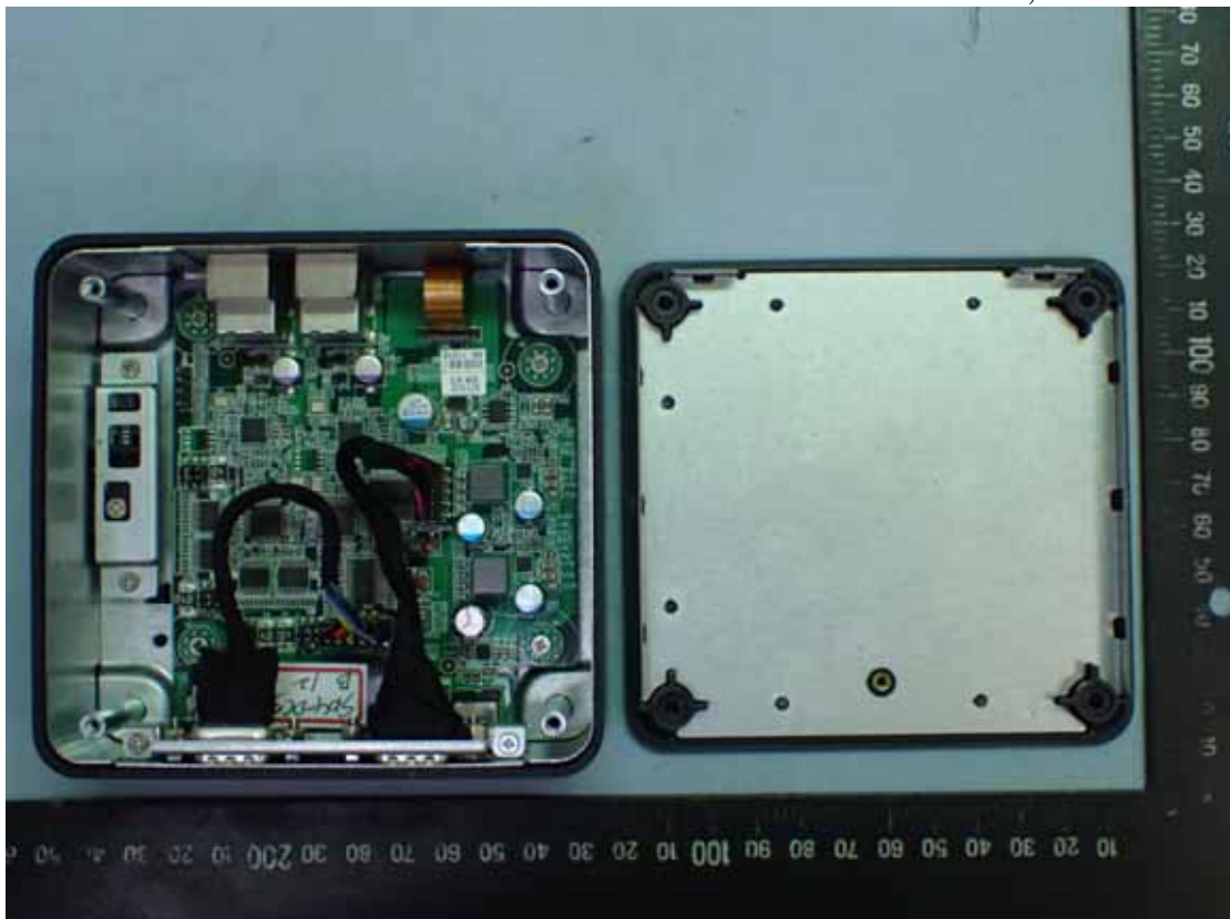
Figure 50 COM Box, Internal View
