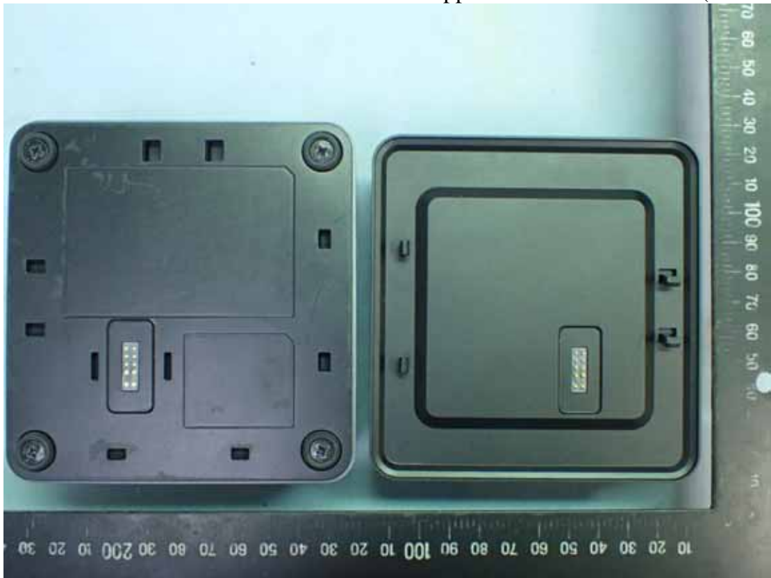
Figure 13 General Appearance with HDD Box (Bottom)
