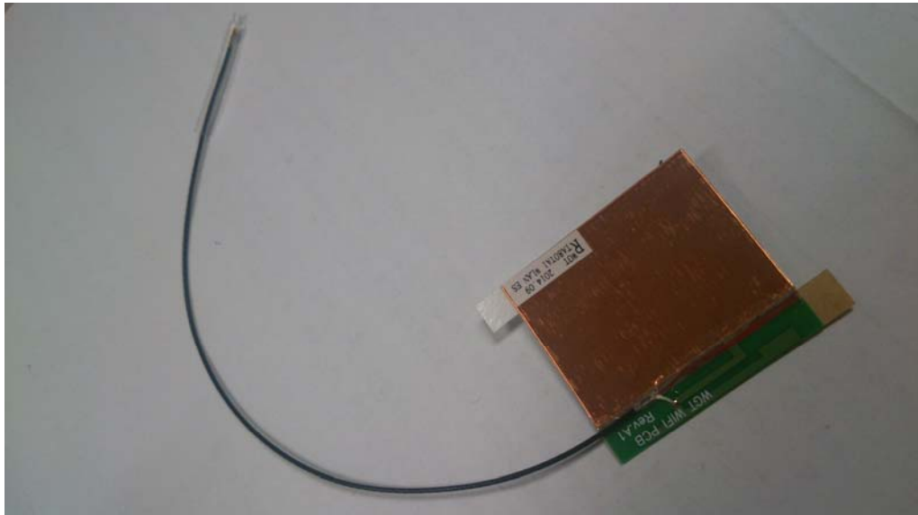
(17) EUT Photo (WLAN+Bluetooth Antenna) (WGT)
