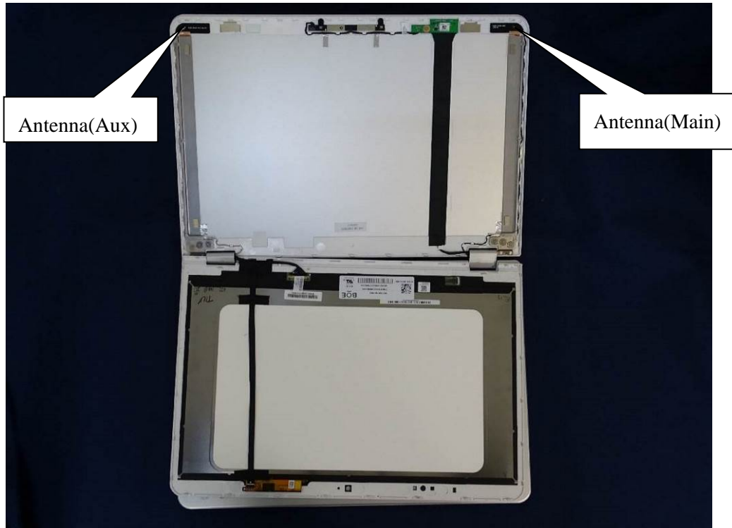
(1) EUT Photo
