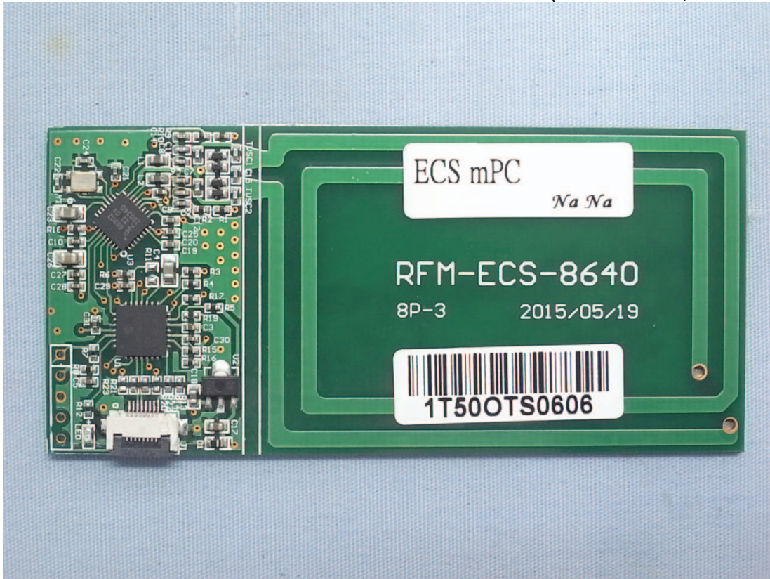
Figure 23 Internal View (NFC Module, Front View)
